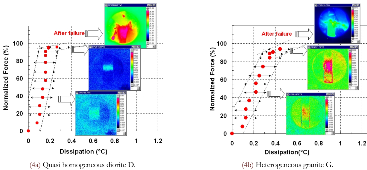
Figure 4: Different stages of heat dissipation describing the process of the damage extent in the granite specimen (characterized by its compressive strength R_c ). Graphical determination of the threshold of acceptable damage TAD of tested materials subject to unconfined loading up to failure.
