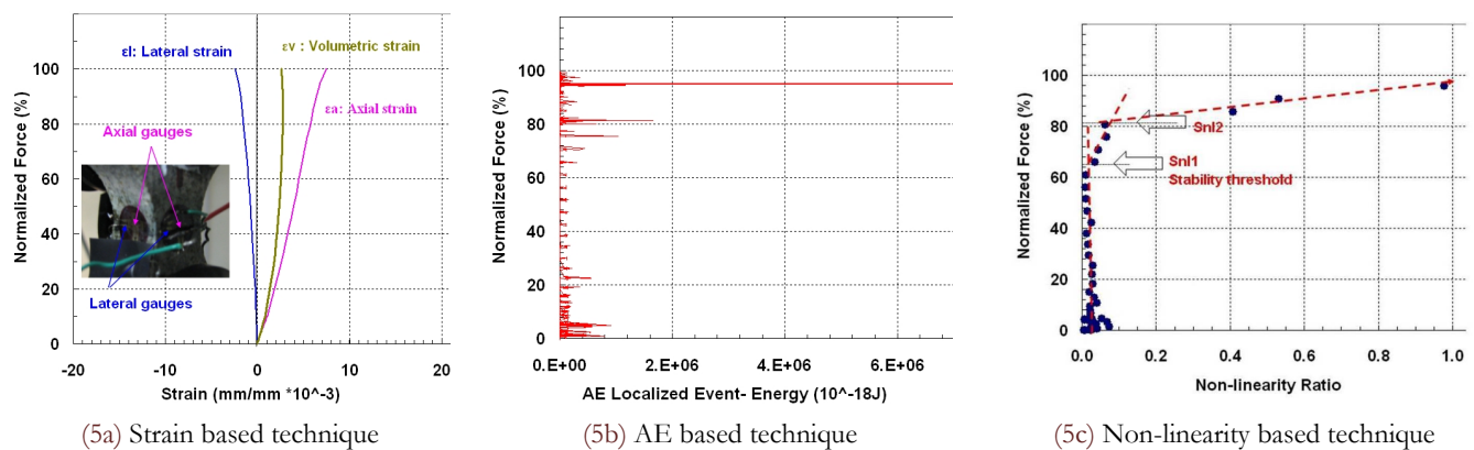
Figure 5: Experimental results obtained when using other testing techniques on granite specimen.
