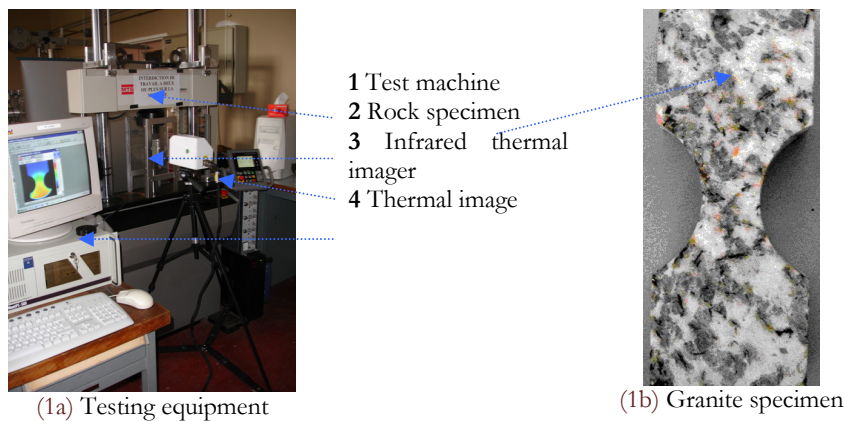
Figure 1: Experimental setup of infrared thermography on a granite specimen.
