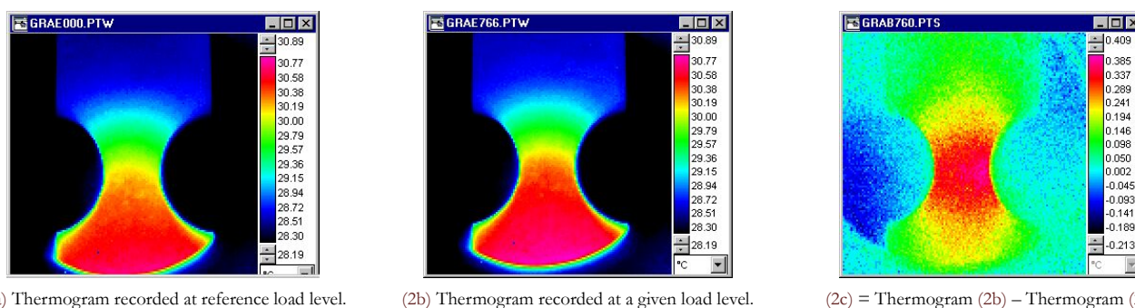
Figure 2: The differential infrared thermography enhances the localization of intrinsic dissipation (temperature changes are given in °C).
