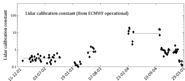
Fig. 4. Time evolution of the actual lidar calibration constant over the period 2002–2005. The horizontal grey lines represent the median of these coefficients.
