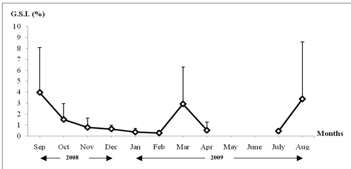
Figure 2: Time evolution of G.S.I. (mean ± standard deviation expressed in %) in male European conger eel ( Conger conger ).
