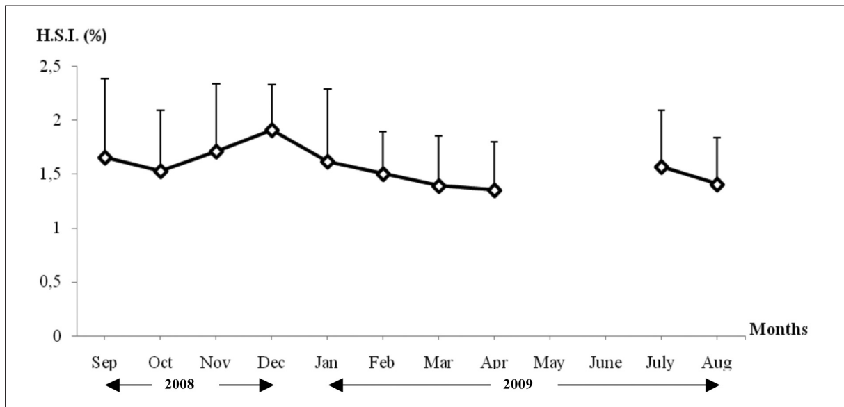
Figure 3: Time evolution of H.S.I. (mean ± standard deviation expressed in %) in male European conger eel ( Conger conger ).
