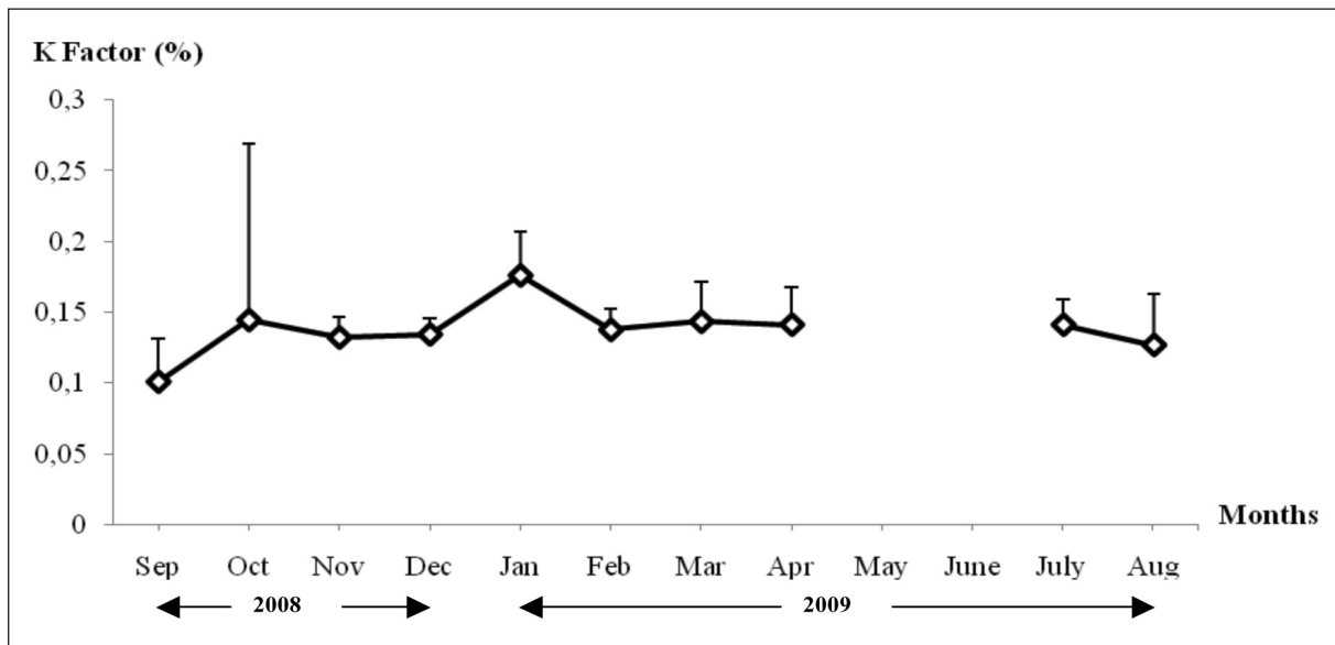
Figure 1: Time evolution of the condition factor K (mean ± standard deviation expressed in %) in male European conger eel ( Conger conger ).
