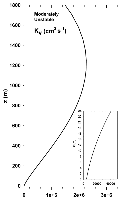
Fig. 3. Eddy diffusivity profile (moderately unstable, h/L = -10 ) used in the Walker Branch Watershed forest canopy simulation for mid-July, 02:00 p.m. LT ( \text{cm}^2 \text{s}^{-1} ). Inset presents K_v profile within the canopy.
