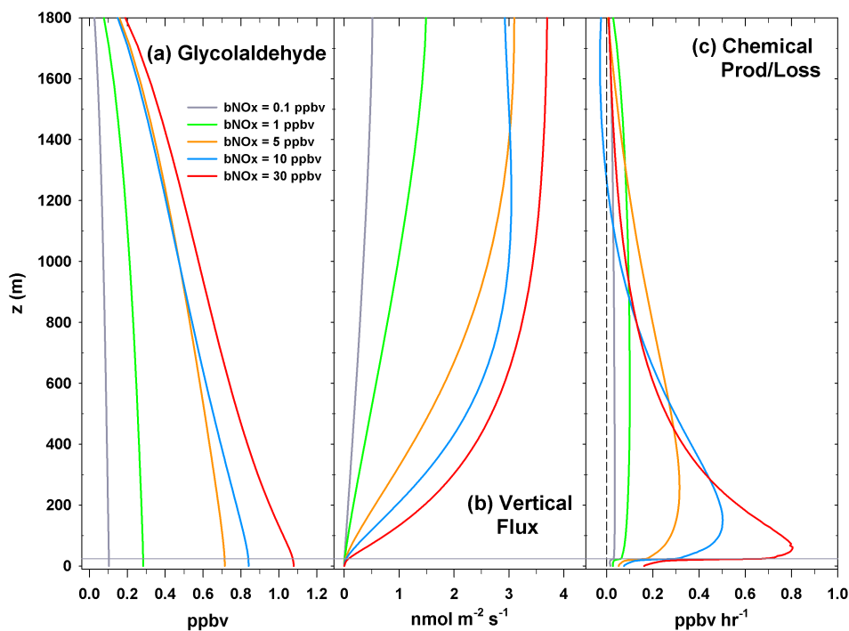
Fig. 13. Vertical profiles of glycolaldehyde (a) mixing ratio (ppbv), (b) vertical flux ( \text{nmol m}^{-2} \text{s}^{-1} ), and (c) chemical production or loss ( \text{ppbv h}^{-1} ) for each background \text{NO}_x value (horizontal gray line is canopy top height).
