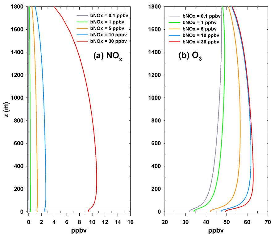
Fig. 6. Steady-state vertical profiles of (a) \text{NO}_x and (b) \text{O}_3 for each background \text{NO}_x value (horizontal gray line is canopy top height).
