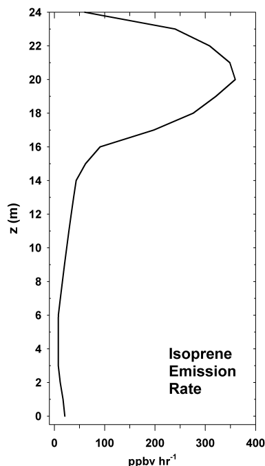
Fig. 4. Isoprene emission rate profile used in the Walker Branch Watershed forest canopy simulation for mid-July, 02:00 p.m. LT ( \text{ppbv h}^{-1} ).
