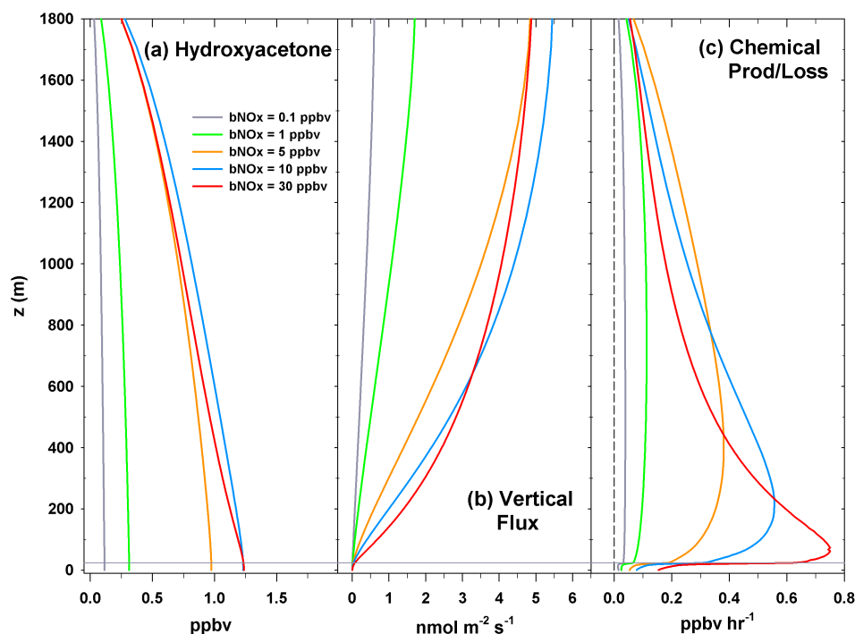
Fig. 14. Vertical profiles of hydroxyacetone (a) mixing ratio (ppbv), (b) vertical flux ( \text{nmol m}^{-2} \text{s}^{-1} ), and (c) chemical production or loss ( \text{ppbv h}^{-1} ) for each background \text{NO}_x value (horizontal gray line is canopy top height).
