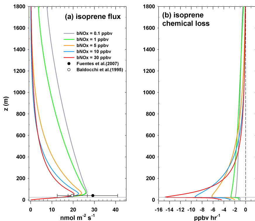
Fig. 8. Steady-state profiles of (a) isoprene vertical flux ( \text{nmol m}^{-2} \text{s}^{-1} ) and (b) isoprene chemical loss ( \text{ppbv h}^{-1} ) for each background \text{NO}_x value (horizontal gray line is canopy top height). Measured isoprene flux data (means \pm 1 standard deviation) from Baldocchi et al. (1995) and Fuentes et al. (2007) for Walker Branch Watershed.
