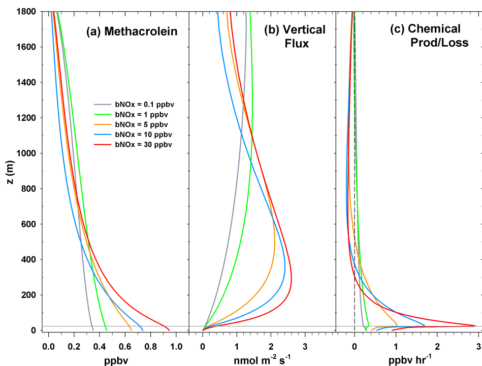
Fig. 9. Vertical profiles of methacrolein (a) mixing ratio (ppbv), (b) vertical flux ( \text{nmol m}^{-2} \text{s}^{-1} ), and (c) chemical production or loss ( \text{ppbv h}^{-1} ) for each background \text{NO}_x value (horizontal gray line is canopy top height).
