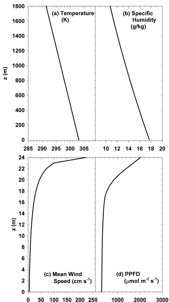
Fig. 2. Input meteorological and radiative flux data used in the Walker Branch Watershed forest canopy simulations for mid-July, 02:00 p.m. LT: (a) air temperature (K); (b) specific humidity ( \text{g kg}^{-1} ); (c) mean wind speed ( \text{cm s}^{-1} ); and, (d) photosynthetic photon flux density ( \mu\text{mol photons m}^{-2} \text{s}^{-1} ).
