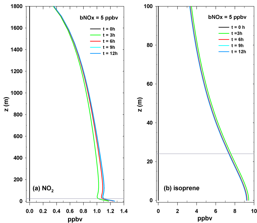
Fig. 5. Vertical profiles of (a) \text{NO}_2 and (b) isoprene for \text{bNO}_x = 5 ppbv, illustrating the approach to steady-state over the 12 h simulation (horizontal gray line is canopy top height).
