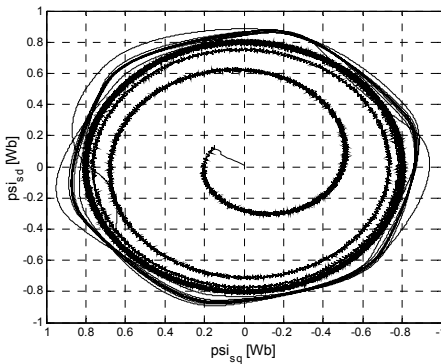
Fig. 11. Stator-flux space-phasor diagram in the stator-fixed reference frame.
