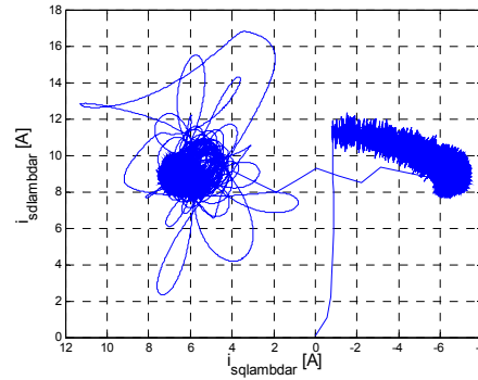
Fig. 5. Stator-current space-phaser diagram in the rotor-field-oriented reference frame.
