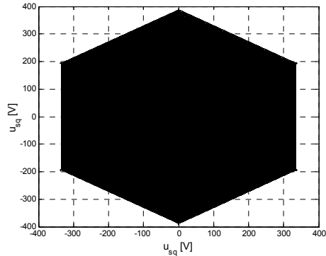
Fig. 15. Stator-voltage space-phasor diagram in the stator-fixed reference frame.
