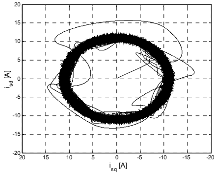
Fig. 9. Stator-current space-phasor diagram in the stator-fixed reference frame.
