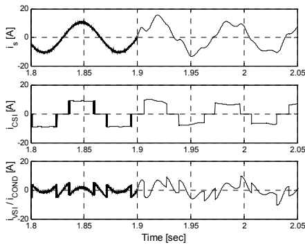
Fig. 10. Motor-, CSI- and VSI/condenser currents before and after the reconfiguration process.
