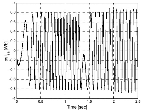
Fig. 13. Stator-flux d component versus time.
