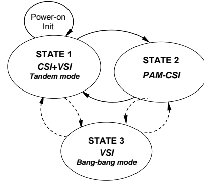
Fig. 2. State machine with three states for the tandem drive.
