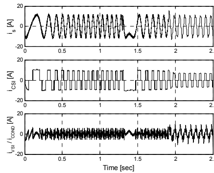
Fig. 6. Current waveforms in a motor phase and at the output of the CSI and VSI/condensers.
