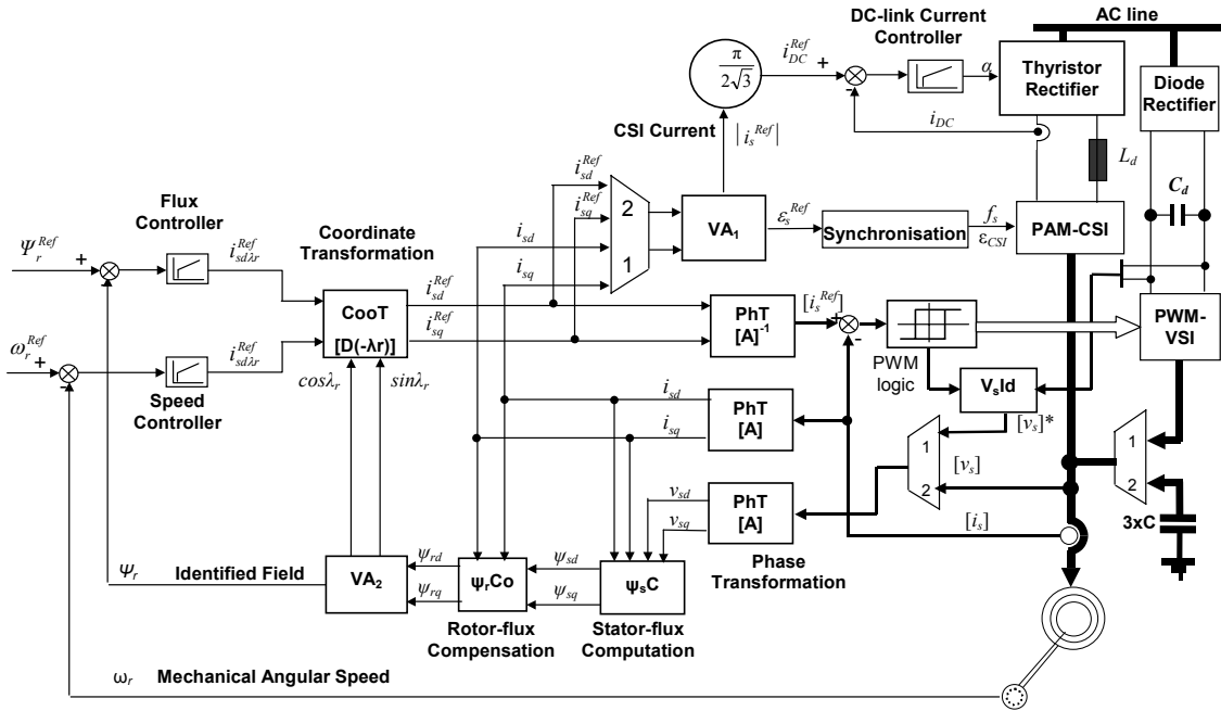
Fig. 1. Reconfigurable vector control structure with two configuration states.
