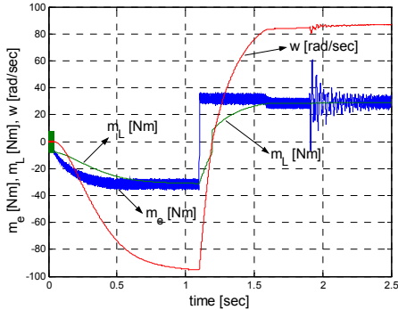
Fig. 3. Rotor electrical-angular speed \omega , electromagnetic- m_e and load-torque m_L versus time.
