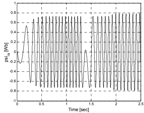
Fig. 14. Rotor-flux d component versus time.
