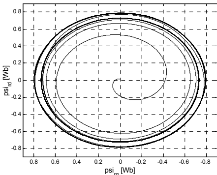
Fig. 12. Rotor-flux space-phasor diagram in the stator-fixed reference frame.
