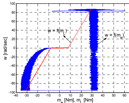
Fig. 4. Motor and load mechanical characteristics during starting, speed reversing and reconfiguration.
