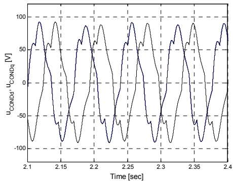
Fig. 16. Condenser-voltage d-q components time diagram after reconfiguration.
