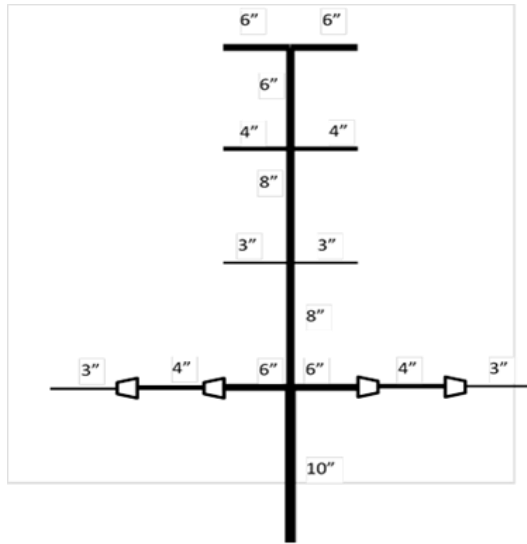
Fig. 7: Piping system to distribute the water
