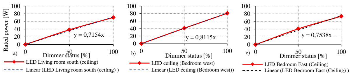
Figure 6. Plot of the Dimmer status-Rated power relationship for the LED installed on the ceiling of a) living room, b) bedroom west and c) bedroom east.
