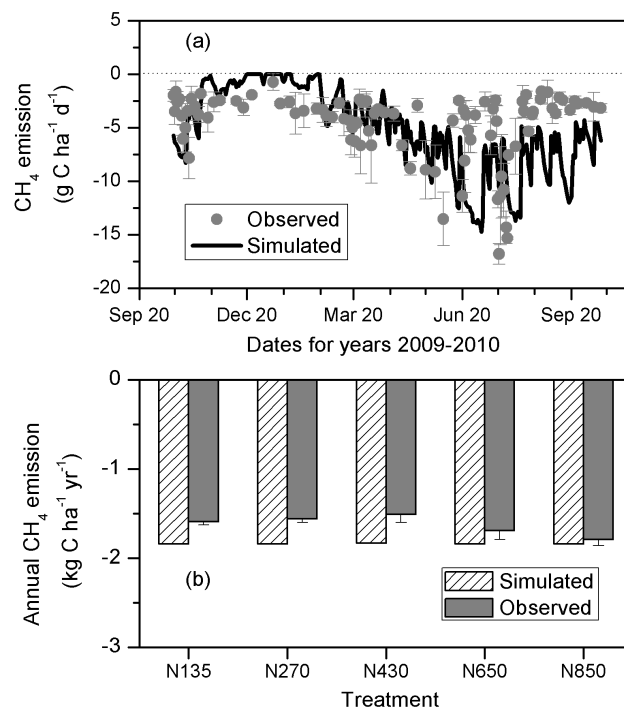
Fig. 5. Observed and simulated daily methane (CH 4 ) fluxes for treatment N430 (a), and cumulative CH 4 emissions (b) for treatments N135, N270, N430, N650 and N850 from 2009 to 2010. Treatment code definitions can be found in Table 1 and in the text. The observed data were adapted from Liu et al. (2012).
