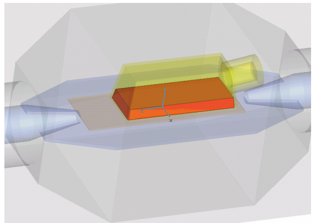
Fig. 4. 3D-model of the so-called \mu TEM cell for exposure of the biological samples to RF radiation under far-field conditions (flask with monolayer of A_L cells plus 5 ml medium on the \mu TEM cell septum) used for numerical evaluation and dosimetry.
