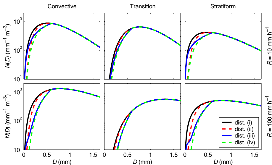
Fig. 5. As Fig. 4, but for simulated 2DVD measurements.
