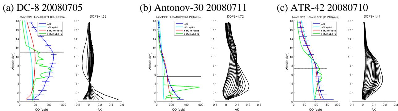
Fig. 8. Same as Fig. 7 for three examples in summer. In situ profiles were measured by the DC-8 on 5 July (a), the Antonov-30 on 11 July (b), and the ATR-42 10 July 2008 (c). See text for details.
