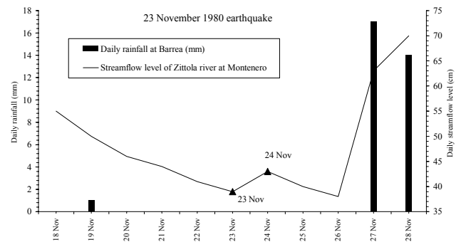
Fig. 5. Hydrological anomaly correlated to the 23 November 1980 earthquake, consisting of an increase in the streamflow rate of Zittola River measured at Montenero, not imputable to rainfalls.
