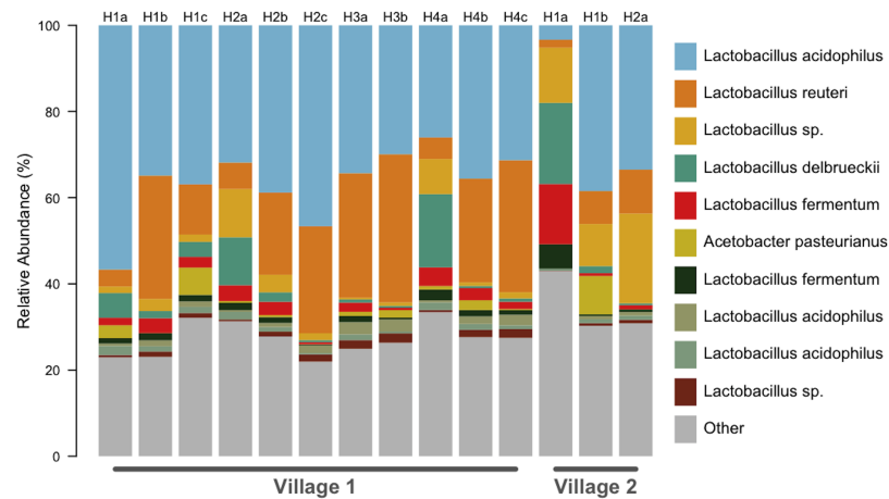
Figure 1 All chicha samples were dominated by Lactobacillus spp. OTU predicted identities are from a manual BLAST search against the NCBI 16S isolate database. We found ten OTUs with greater than 1% relative abundance. This barplot shows the relative abundance (%) of ten most common bacteria isolates for each sample. Up to three independent batches were sampled for each house (e.g., H1a–H1c). Eleven samples were analyzed from Village 1 and three from Village 2.
