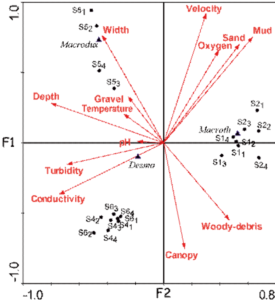
Figure 2 Canonical correspondence analysis triplot showing species and sampling stations in relation to environmental variables in Banco River Basin: Macrothysi = Macrobrachium thysi ; Macrodux = Macrobrachium dux ; Desmo = Desmocaris trispinosa ; station (S); number of station (1–6); sampling period in indices (1 = May, 2 = September, 3 = October, 4 = February).
