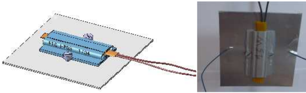
Figure 3. HP03 1/04 thermistor mounted on aluminium plate
