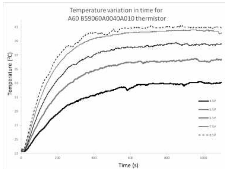
Figure 6. Temperature variation for A60 B59060A0040A010
