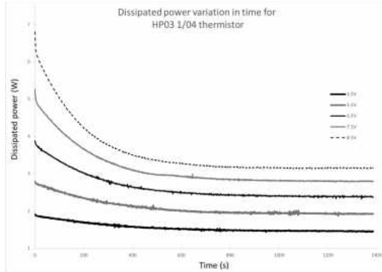
Figure 9. Power dissipation variation for HP03 1/04
