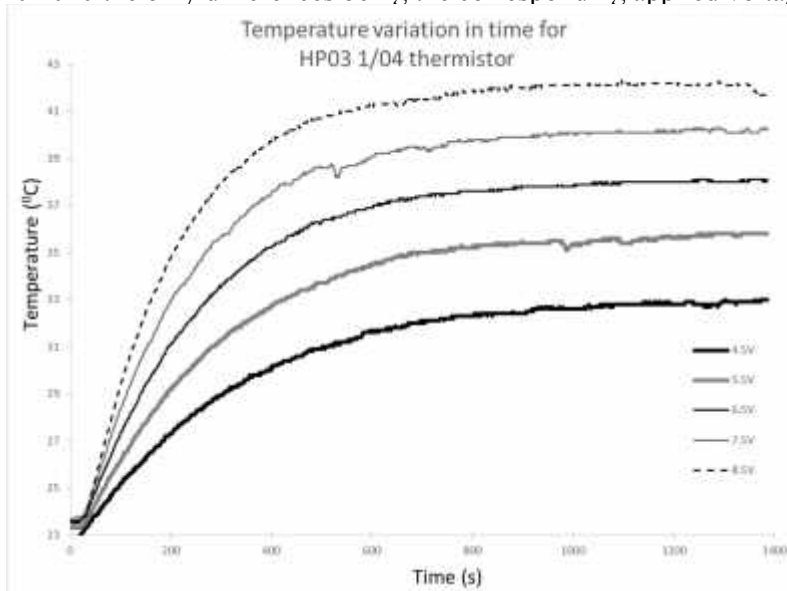
Figure 8. Temperature variation for HP03 1/04
