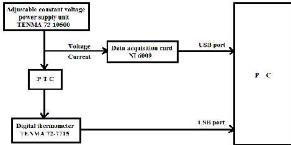
Figure 1. Block diagram of the measurement system
