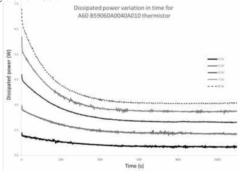
Figure 7. Power dissipation variation for A60 B59060A0040A010
