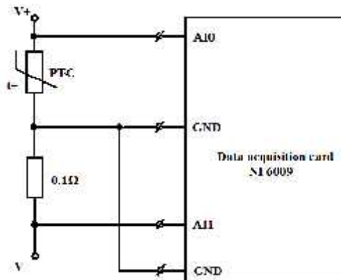
Figure 5. Circuit diagram for PTC testing
