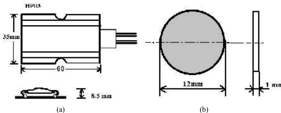
Figure 2. PTC dimensions HP03 1/04 (a) and A60 B59060A0040A010 (b)
