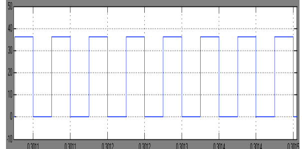
Fig.4.e.Voltage across the switch SR2.
