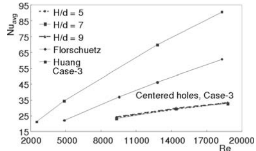
Figure 10. Comparison of average Nusselt number of present study with other studies for different jet Reynolds number and for different feed channel aspect ratios (for orifice jet-plate with centered holes, outflow in both directions)
