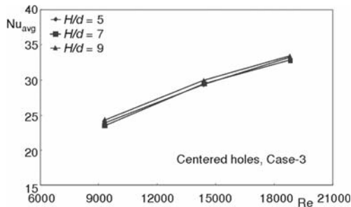
Figure 9. Average Nusselt number distribution for different jet Reynolds number and for different feed channel aspect ratios (for jet-orifice plate with centered holes, for outflow passing out in both directions – Case-3)
