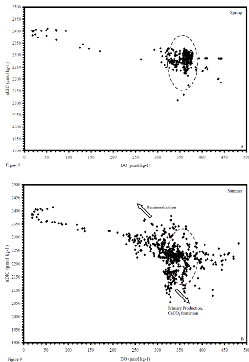
Fig. 9. Spring and summer concentrations of nDIC ( \mu\text{moles kg}^{-1} ) relative to spring and summer concentrations of DO ( \mu\text{moles kg}^{-1} ) (A) Spring. Most points clustered within the highlighted area of DO concentrations between 300 and 400 \mu\text{moles kg}^{-1} , and DIC concentrations between \sim 2200 and 2450 \mu\text{moles kg}^{-1} . (B) Summer. DIC concentrations were much less clustered and mostly lower relative to DO concentrations in spring. For ease of comparison, the springtime cluster is also shown in this figure (highlighted area). The arrows show the effects of primary production and carbonate mineral dynamics between station occupations: NCP draws values down and to the right, as surface layer DIC is consumed and DO is produced; remineralization draws values up and to the left as DIC is produced and DO is consumed.
