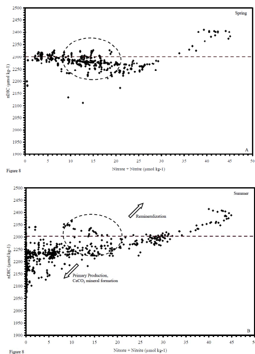
Fig. 8. Spring and summer concentrations of nDIC ( \mu\text{mol kg}^{-1} ) relative to nitrate+nitrite ( \mu\text{mol kg}^{-1} ). (A) Spring. For nearly all concentrations of nitrate+nitrite, nDIC ranged from \sim 2225 \mu\text{mol kg}^{-1} to 2350 \mu\text{mol kg}^{-1} . Average spring concentration ( 2300 \mu\text{mol kg}^{-1} ) is marked by the dotted line. (B) Summer. nDIC concentrations decreased with respect to nitrate, ranging from \sim 2050 \mu\text{mol kg}^{-1} to 2350 \mu\text{mol kg}^{-1} . The springtime average ( 2300 \mu\text{mol kg}^{-1} ) is also plotted here, showing that most summertime points fall below the springtime average due to primary production and carbonate mineral formation.
