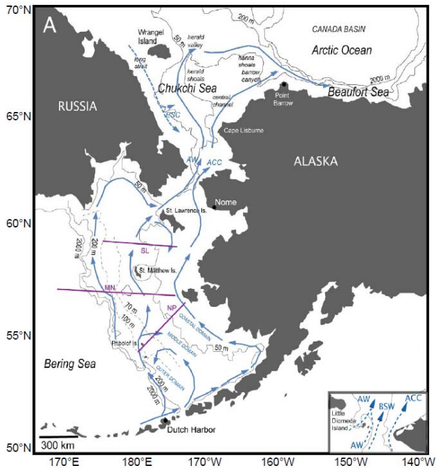
Fig. 1. Map of the Bering Sea showing the locations of the three domains, Outer Middle and Coastal. The locations of the three east-west transect lines (SL, MN, and NP) are also shown as well as the general circulation. During the winter, sea-ice covers much of the Bering Sea shelf, but the advance is constrained by the presence of relatively warm water in the central and southern Bering Sea. During winter, water-masses are confined to a small range of temperature-salinity through mixing and homogenization by ventilation, brine rejection and mixing. During the summertime, sea-ice retreats into the Chukchi Sea and Canada Basin of the Arctic Ocean.
