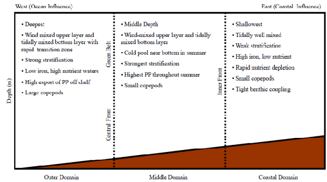
Fig. 2. Biogeochemical features of the Outer, Middle, and Coastal domains of the Bering Sea Shelf.
