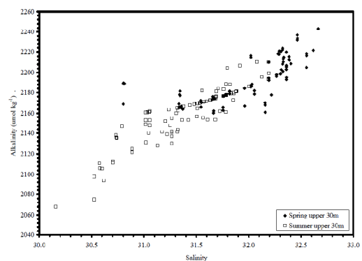
Fig. 10. Spring and summer concentrations of TA ( \mu\text{moles kg}^{-1} ) in the upper 30 m of the water column. Overall, TA concentrations were lower in summer than in spring, although some summer values were higher. This seasonal change necessitates the application of a correction factor to NCP estimates which accounts for the formation and dissolution of TA.
