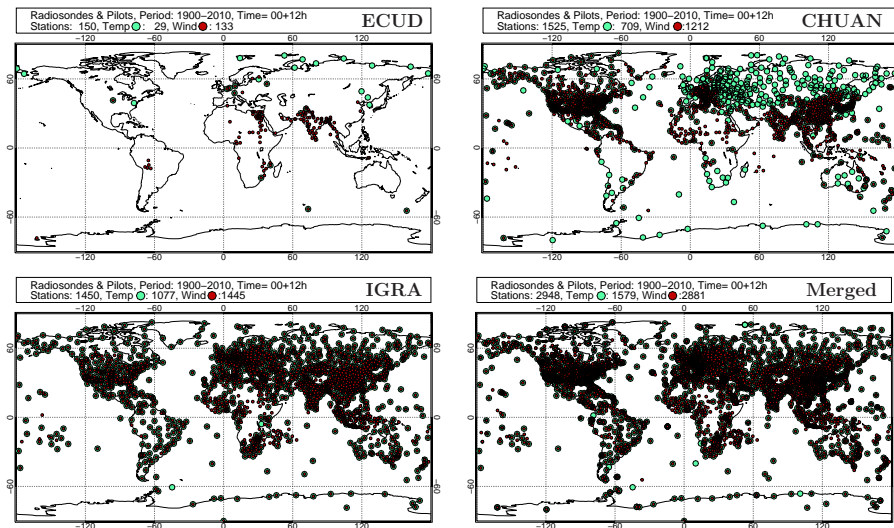
Figure 2. Spatial distributions of stations with at least 365 days of data, at the pressure levels of 850, 700 and 500 hPa, in the different data sets used in this study. The bottom right panel shows the distribution in the merged archive. Only WMO stations have been used.
