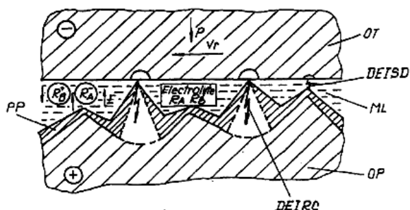
Fig.1. The fundamental scheme of processing through complex erosion
