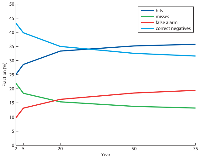
Fig. 7. Comparison of percentage of hits, misses, false alarms and correct negatives (definition in Table 1) for the 20 largest catchments on the globe and different return periods (areas which contain no data in the benchmark are masked). This compares the maps computed in this study to the data of the benchmark study.
