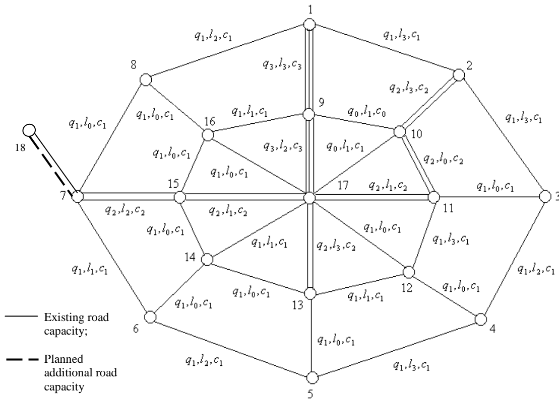
Fig. 2. Simple radial-circular street network ( q_i – capacity, l_i – length, c_i – cost function)
