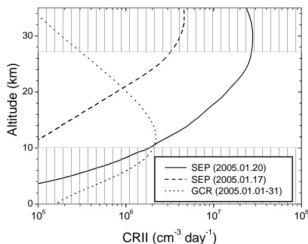
Fig. 1. Daily integrated cosmic ray induced ionization (CRII) of the polar atmosphere in January 2005. Solid and dashed curves depict the net ionization due to two SEP events, of 20 January and 17 January (a typical event), respectively. The dotted curve depicts the average ionization rate due to galactic cosmic rays in January 2005.
