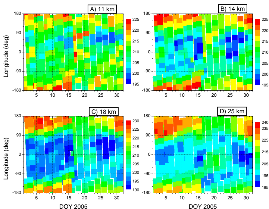
Fig. 6. Temperature distribution in the Northern Polar stratosphere as a function of geographical longitude and time, for four fixed altitudes as indicated on top of each panel. Color scale is shown to the right of each panel.
