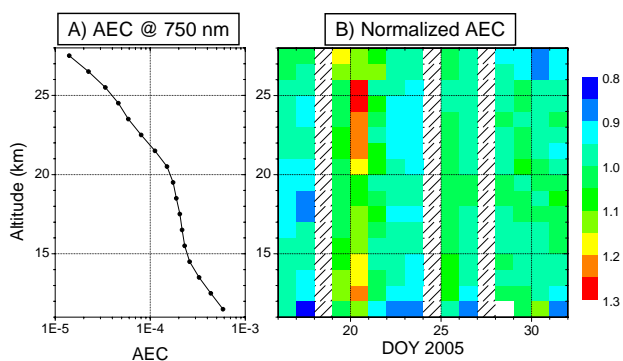
Fig. 7. Averaged OSIRIS aerosol extinction (in \text{km}^{-1} ) profiles at 750 nm measured over the Antarctic region in the second half of January 2005. (A) The average profile for the 16–31 January 2005 period. (B) Normalized (to that shown in A ) daily averaged AEC. Hatched area depicts days with no data available.
