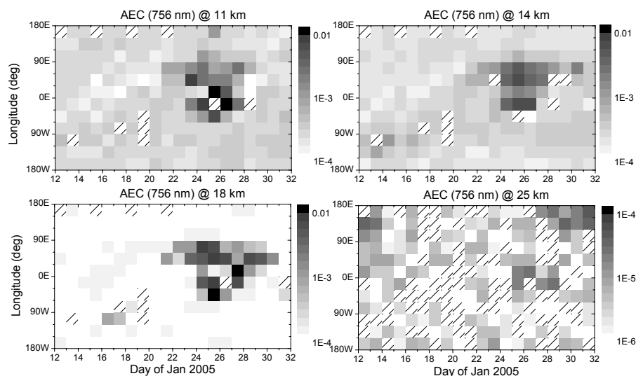
Fig. 3. Daily averaged aerosol extinction coefficient (in \text{km}^{-1} ) at the 756 nm wavelength measured by SAGE III instrument at fixed altitudes (as denoted on top of each panel) as a function of geographical longitude. Logarithmic grey scale is shown on the right of each panel.
