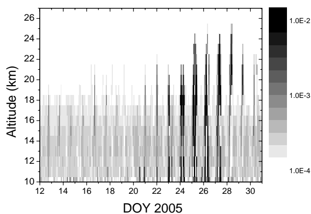
Fig. 2. Vertical profiles of aerosol extinction coefficient (in \text{km}^{-1} ) at the 756 nm wavelength measured by SAGE III in the Northern Polar region (zonal mean, 66\text{--}72^\circ\text{N} ) during 13–30 January 2005. Logarithmic grey scale is shown on the right panel.
