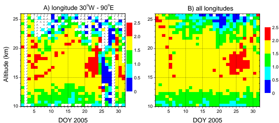
Fig. 5. Ångström exponent \alpha calculated from SAGE III aerosol extinction as a function of altitude and time. Data were averaged over the longitudinal region 30^{\circ} W– 90^{\circ} E (A) and all longitudes (B) in the Northern Polar region (latitude 66^{\circ} – 73^{\circ} ).
