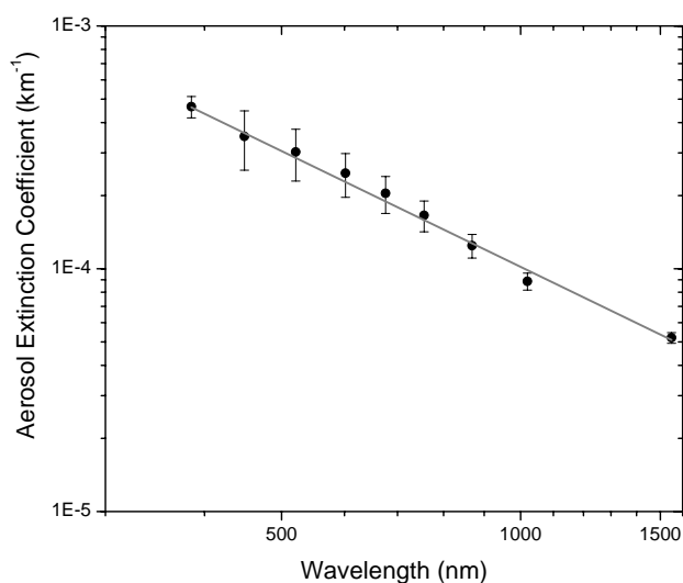
Fig. 4. An example of wavelength dependence of SAGE aerosol extinction coefficients (1 January 2005 at height 15.25 km). Solid line corresponds to the best fit power law (Ångström exponent) \alpha = 1.58 \pm 0.05 .
