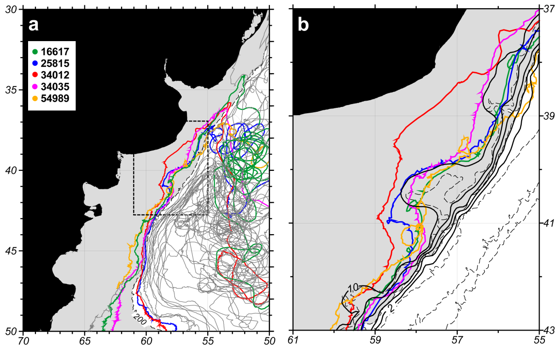
Fig. 10. Trajectories of WOCE surface drifters in the western South Atlantic. (a) All observed drifters in grey, color tracks indicate drifters exhibiting relatively sharp inshore loops near 41^{\circ} S. The light shading marks waters shallower than 200 m. (b) Expanded view of the region indicated by the dashed rectangle in (a) with color drifter tracks overlapped with lines of constant potential vorticity (black contours in 10^{-7} \text{ m}^{-1} \text{ s}^{-1} ). The dashed lines in (b) are the 100, 200 (shaded), 1000, 2000 and 3000 m isobaths from GEBCO.
