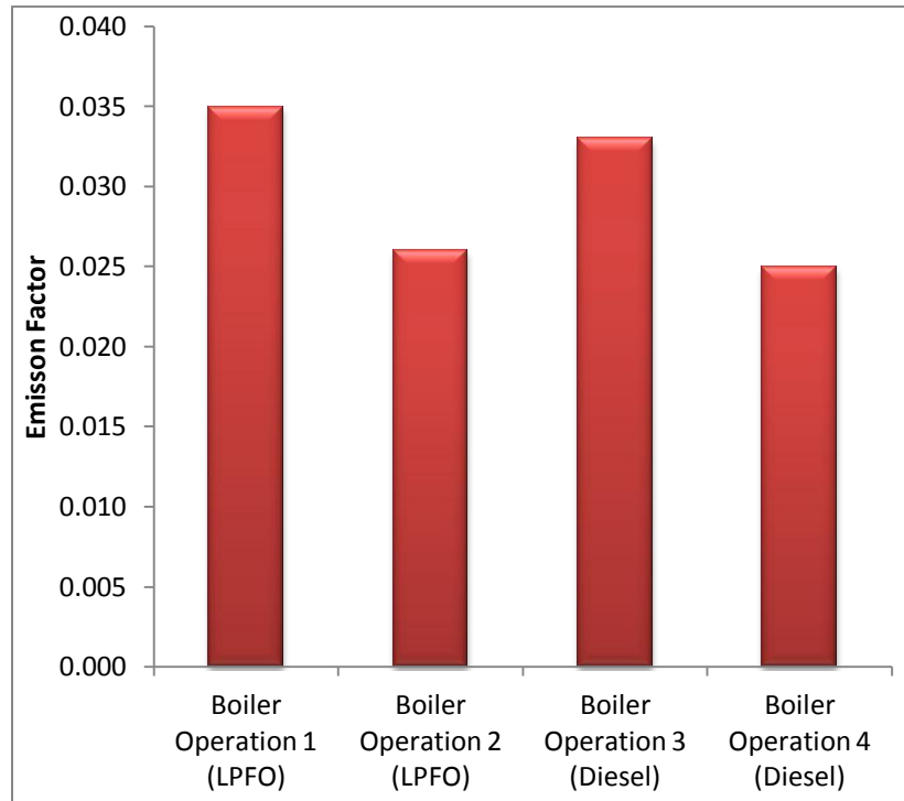
Figure 2. Emission factor of water vapour in the boilers
