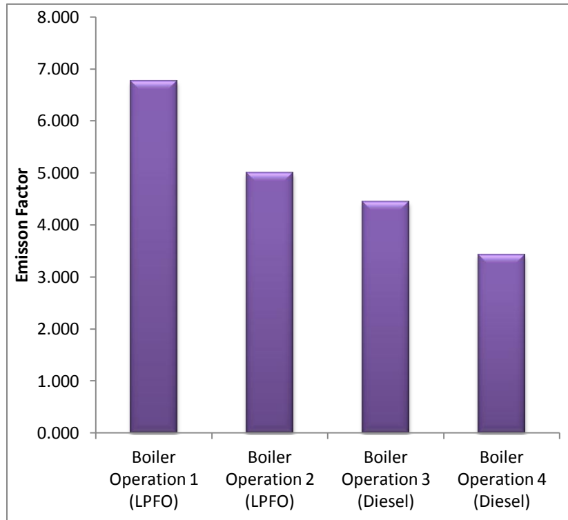
Figure 4. Emission factor of nitrogen in the boilers
