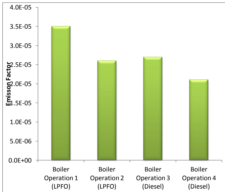
Figure 3. Emission factor of Sulphur dioxide in the boilers
