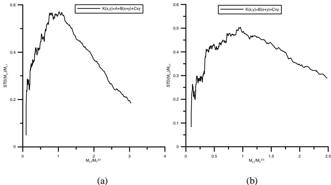
Fig. 9. The ratio of the standard deviation to expectation value of the largest droplet \text{STD}(M_{L1})/M_{L1} as a function of M_{L1}/M_T^{2/3} for approximating polynomials (a) A+B(x+y)+Cxy and (b) B(x+y)+Cxy .
