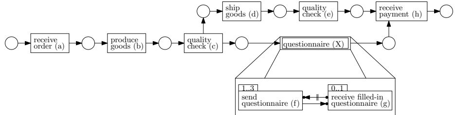
Fig. 7. Hybrid model of a basic order-fulfilment process.
