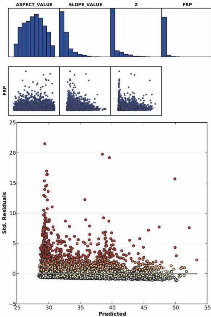
Figure 8. Histograms and Scatterplots of Ordinary Least Square linear regression showing variable distribution and relationships, and residual vs. predicted plot for FRP as dependant and aspect, slope and elevation as explanatory variable
