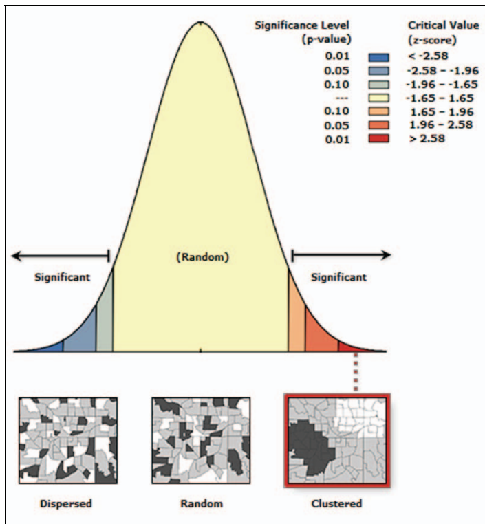
Figure 6. Global Moran's I Spatial autocorrelation results
