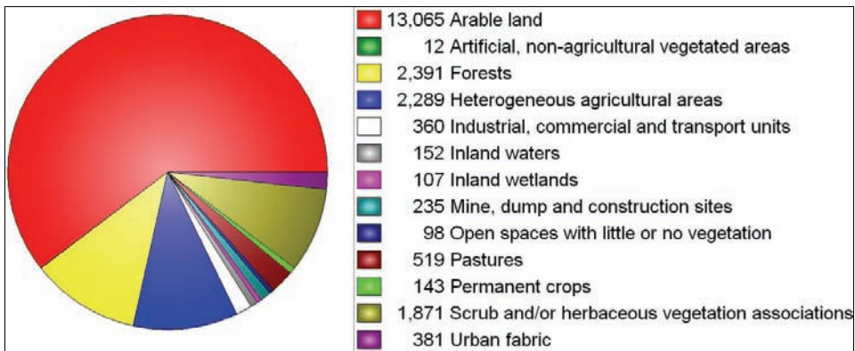
Figure 1. Number of fires per CORINE Land Cover level 2 for period November 2000 – August 2013
