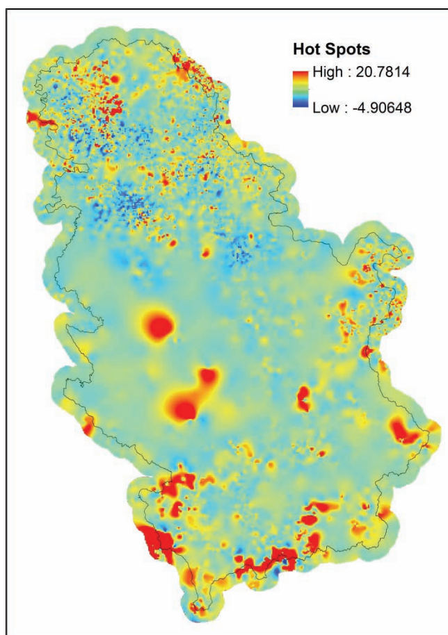
Figure 5. Getis-Ord G_i^* Hot Spots of FRP interpolated to surface
