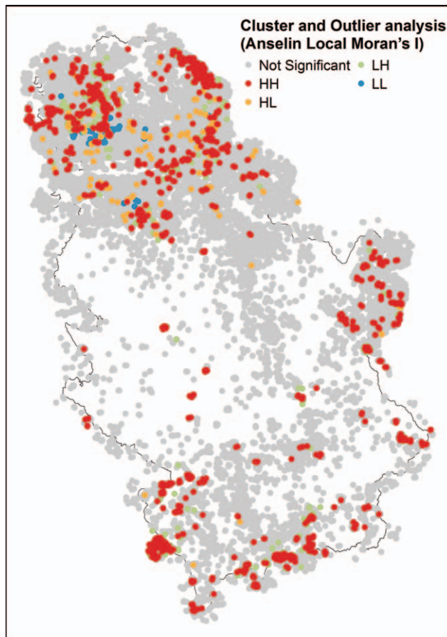
Figure 7. Anselin Local Moran's I Cluster and Outlier analysis results
