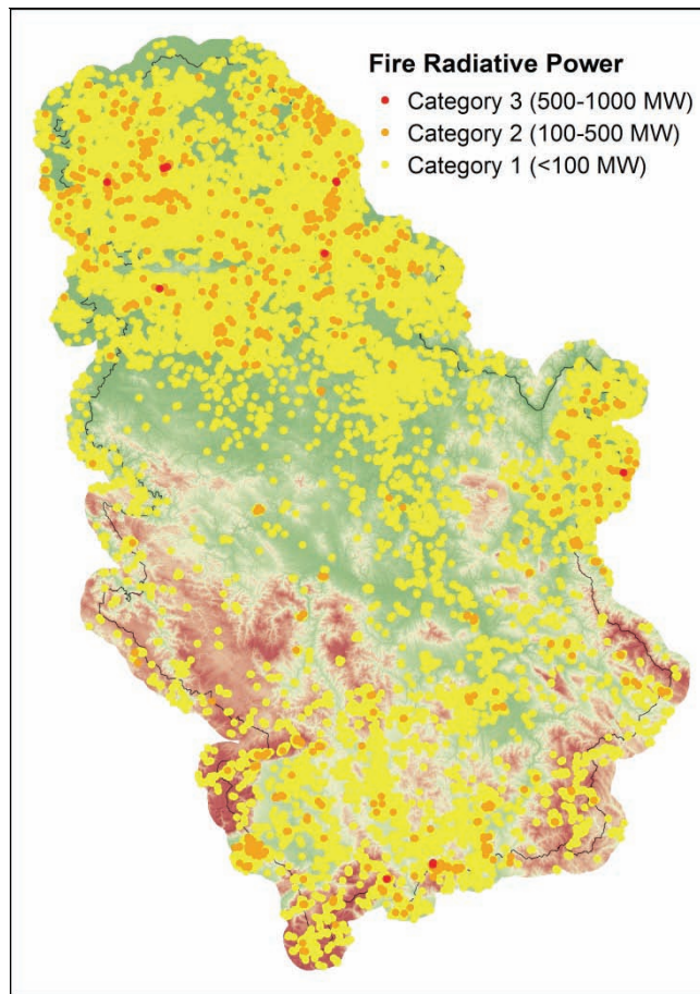
Figure 4. Geographical distribution of fires and Fire Radiative Power in Serbia for period November 2000-August 2013
