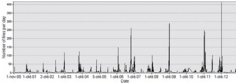
Figure 2. Frequency of fires per day for period November 2000 – August 2013
