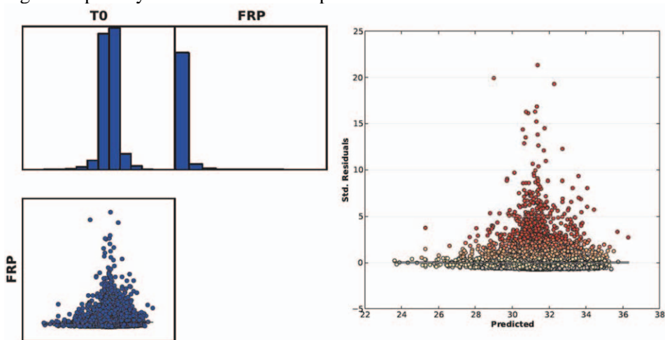
Figure 9. Histograms and Scatterplots of Ordinary Least Square linear regression showing variable distribution and relationships, and residual vs. predicted plot for FRP as dependant and total solar radiation as explanatory variable
