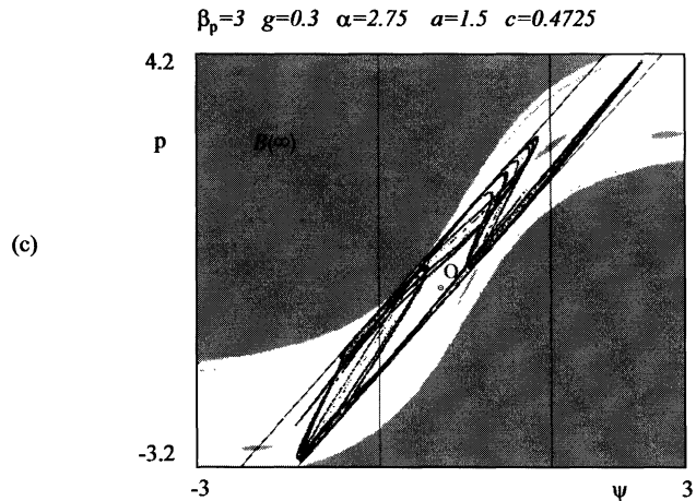
FIGURE 6 A different example of a chaotic attractor of annular shape, obtained for \beta_p=3 , g=0.3 , \alpha=2.75 , a=1.5 , c=0.4725 : the basin of the attractor is the white area, while the grey points have divergent trajectories. The presence of only few “holes” is due to the fact that arcs on the boundary of B(\infty) have “just” crossed the critical curve LC .
