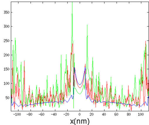
Figure 9: Intensity of the electric field |E|^2 inside the nanoantenna (—: biosensor with smooth surface, —: biosensor with rms roughness 0.82 nm and —: biosensor with rms roughness 1.41 nm; the gap between the two nanorods is from x = -10 to x = 10 nm)
