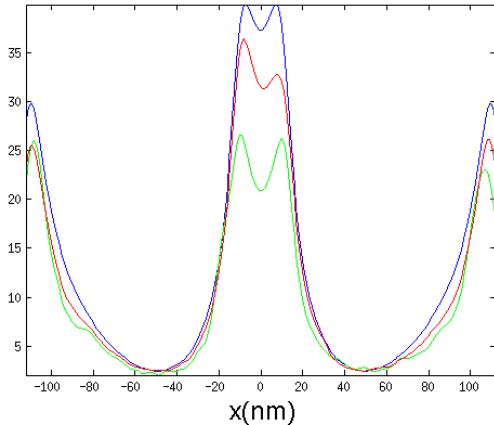
Figure 11: Intensity of the electric field |E|^2 at 6 nm above the nanoantenna (—: biosensor with smooth surface, —: biosensor with rms roughness 0.82 nm and —: biosensor with rms roughness 1.41 nm; the gap between the two nanorods is from x = -10 to x = 10 nm)
