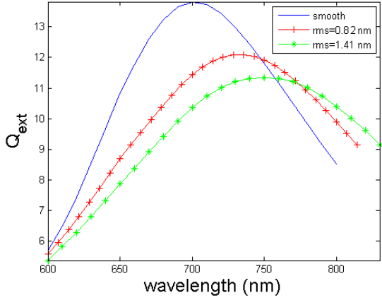
Figure 6: Extinction efficiency spectra of nanoantenna-based biosensor for smooth (blue curves) and rough topography.
