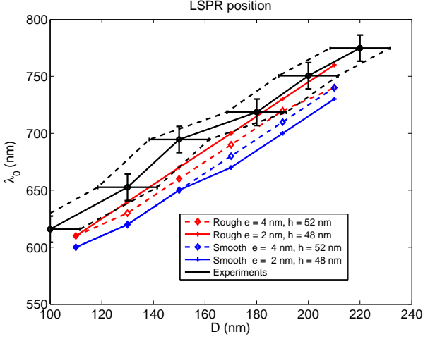
Figure 4: Experimental data from [25] with standard uncertainties. Intervals for the position of the LSPR computed with DDA, using experimental uncertainties, for smooth and rough nanostructures.
