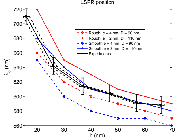
Figure 5: Experimental data from [26] with standard uncertainties. Intervals for the position of the LSPR computed with DDA, using experimental uncertainties, for smooth and rough nanostructures.
