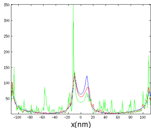
Figure 10: Intensity of the electric field |E|^2 at 3 nm above the nanoantenna (—: biosensor with smooth surface, —: biosensor with rms roughness 0.82 nm and —: biosensor with rms roughness 1.41 nm; the gap between the two nanorods is from x = -10 to x = 10 nm)
