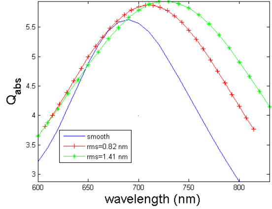
Figure 7: Absorption efficiency spectra of nanoantenna-based biosensor for smooth (blue curves) and rough topography.
