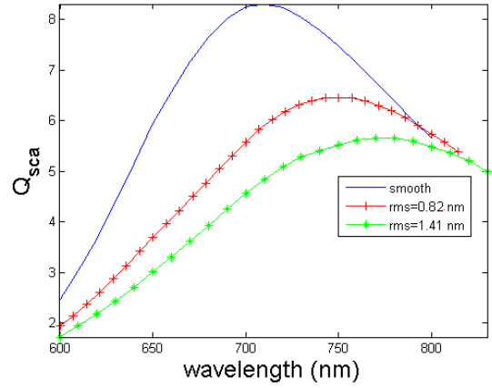
Figure 8: Scattering efficiency spectra of nanoantenna-based biosensor for smooth (blue curves) and rough topography.
