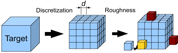
Figure 1: The basic idea of DDA: discretizing the target in a set of dipoles, and roughness control.
