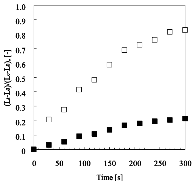
Figure 4. Relative swelling of microphase-separated self-oscillating gel and poly(NIPAAm- co -Ru(bpy) 3 ) gels, (L_t - L_0)/(L_e - L_0) , in the solution of 5 mM Ce(SO 4 ) 2 , 0.894 M HNO 3 at 18 °C as functions of the time t elapsing after changing the solution. L_t , L_0 and L_e , are the lengths of the gel at t = t , initial state and equilibrium state. (□) microphase-separated self-oscillating gel; (■) poly(NIPAAm- co -Ru(bpy) 3 ) gel. S. Maeda et al. Peristaltic motion of polymer gels. Angew. Chem. Int. Ed. 2008 , 47 , 6690-6693. Copyright Wiley-VCH Verlag GmbH & Co.KGaA. Reproduced with permission.
