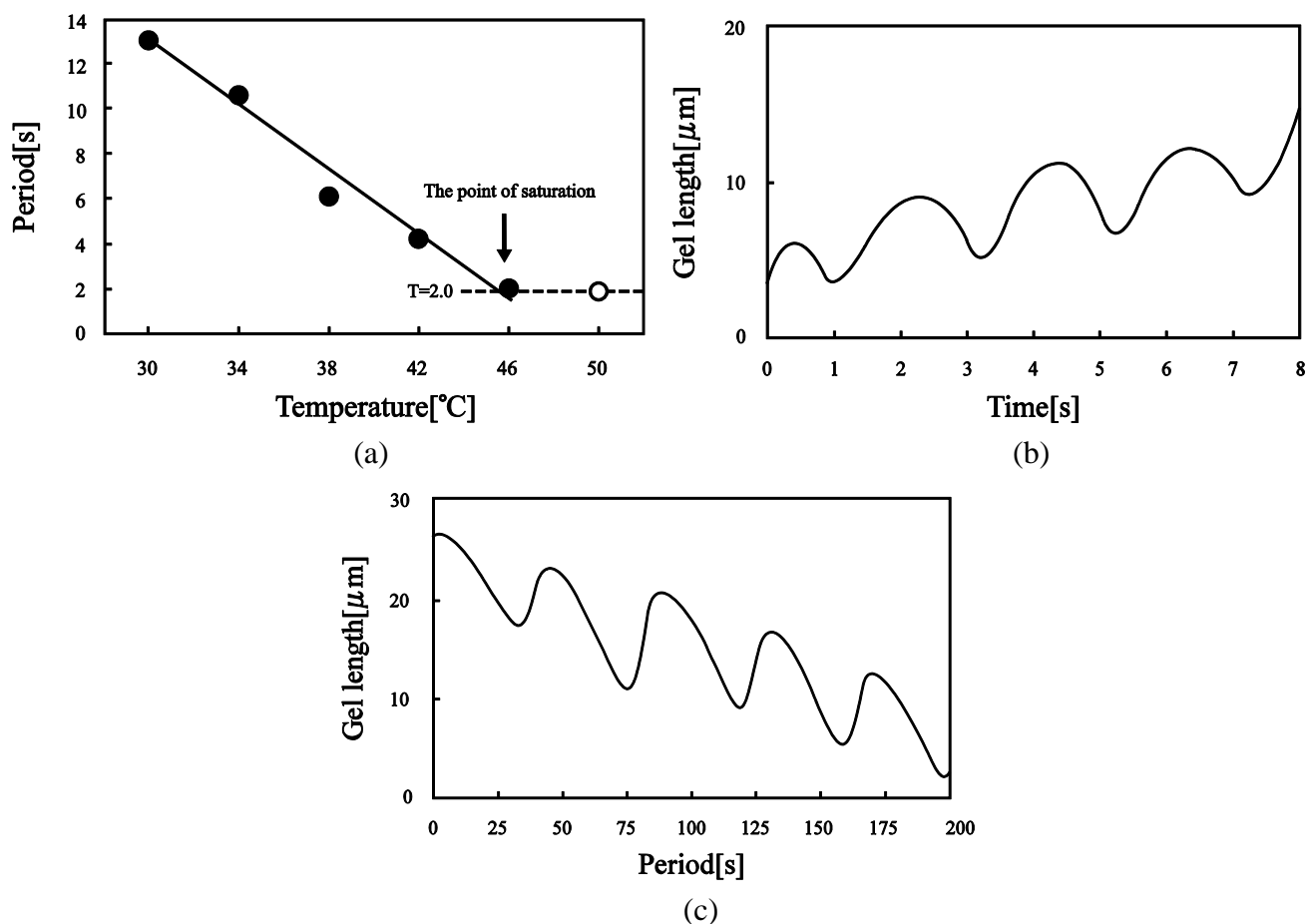
Figure 9. (a) Dependence of the self-oscillation period on the temperature. (●) plots and (○) plots show the linear relation and the saturated line vs. temperature, respectively. (b) Self-oscillating profile of cubic poly(VP-co-Ru(bpy) 3 ) gel at 50 °C (MA = 0.08 M, NaBrO 3 = 0.48 M and HNO 3 = 0.48 M). (c) Self-oscillating profile of cubic poly(VP-co-Ru(bpy) 3 ) gel at 20 °C (MA = 0.08 M, NaBrO 3 = 0.48 M and HNO 3 = 0.48 M). Cubic gel (each side length is about 2 mm and 20 mm) was immersed in 8 mL of the mixture solution of the BZ substrates. Reprinted from Ref. [33] with permission; © The American Chemical Society.
