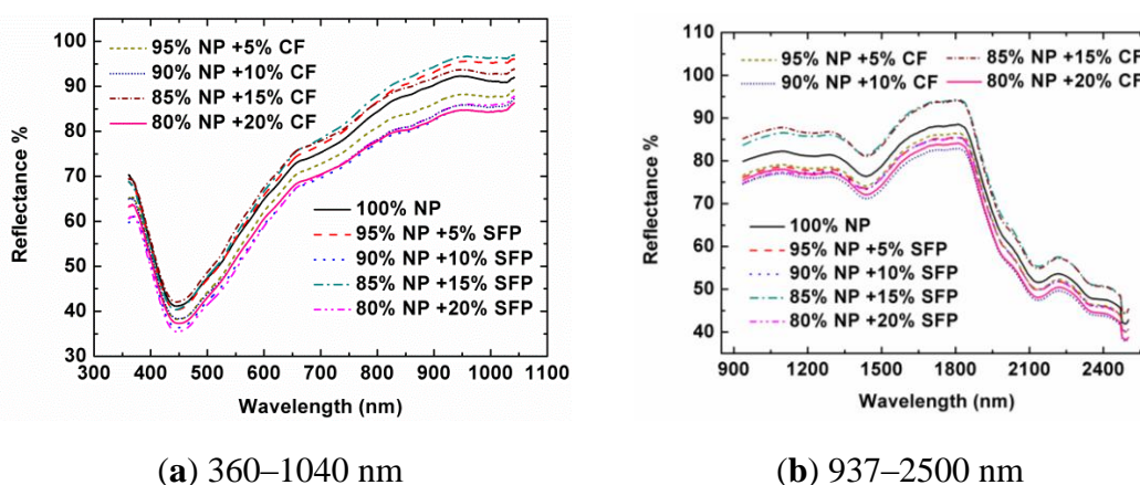
Figure 1. Spectral patterns of the tested notoginseng powder (NP) adulterated by different concentrations of sophora flavescens powder (SFP) and/or corn flour (CF) in 360–1,040 nm (a) and 937–2,500 nm (b). Percentages are shown by mass (g/g).
