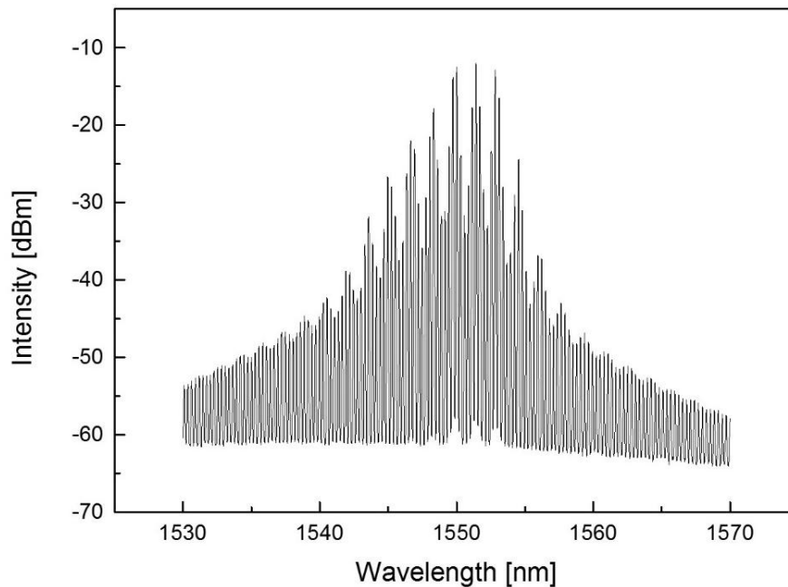
Figure 3. The spectrum of the FP-LD used for Rayleigh OTDR.
