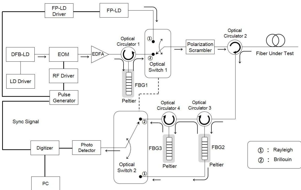
Figure 4. Schematic diagram of the developed OTDR and BOTDR systems.
