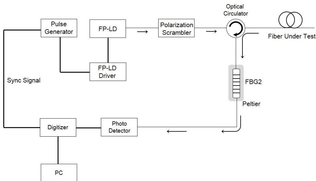
Figure 2. Schematic diagram of Rayleigh OTDR.
