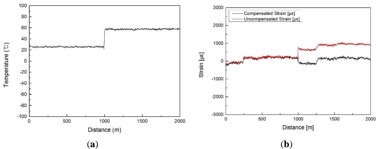
Figure 8. Distributed (a) temperature and (b) strain profiles measured from the developed BOTDR system.
