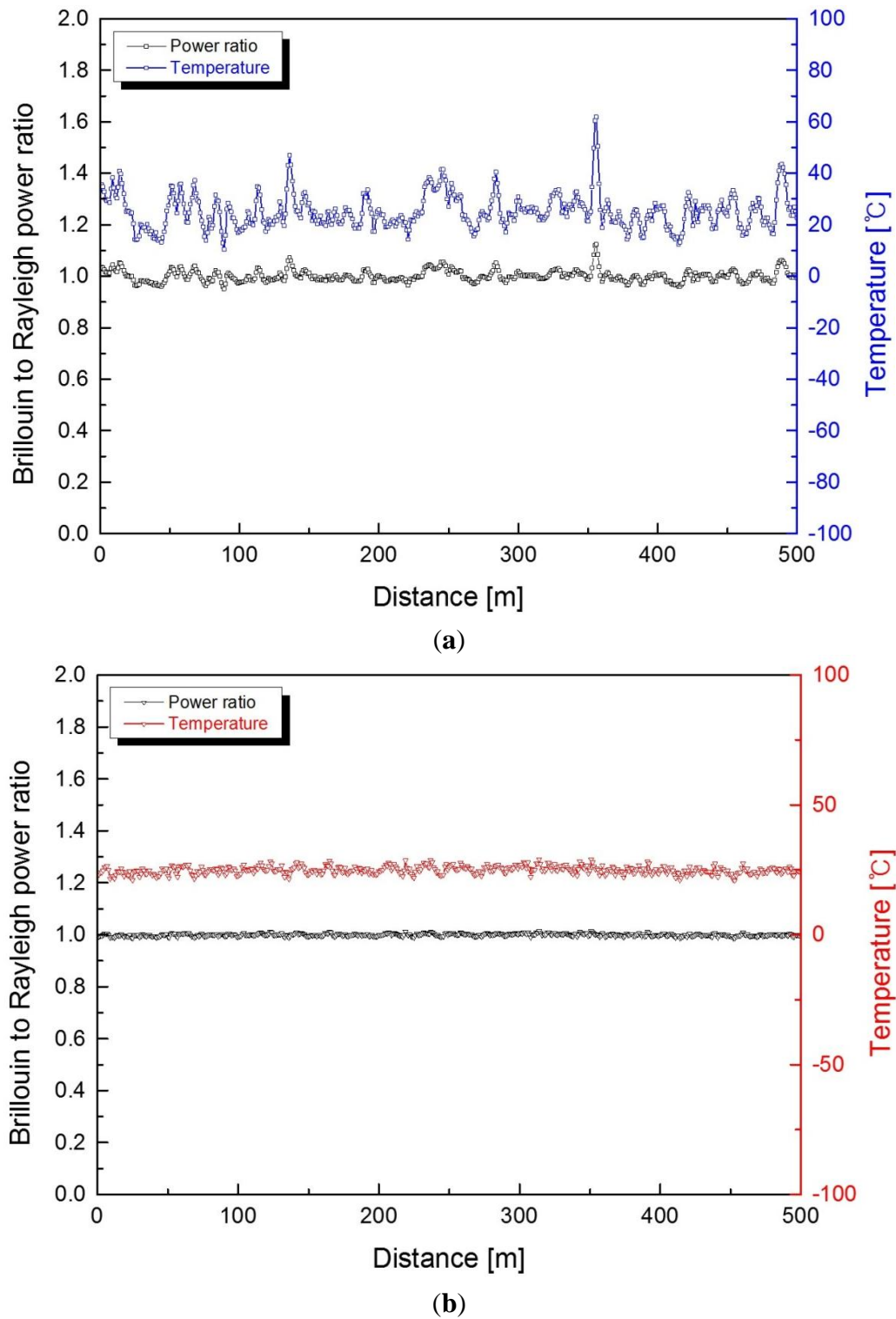
Figure 6. Measured Brillouin to Rayleigh power ratio and distributed temperature profiles for (a) the single-stage and (b) the dual-stage FBG demultiplexer.
