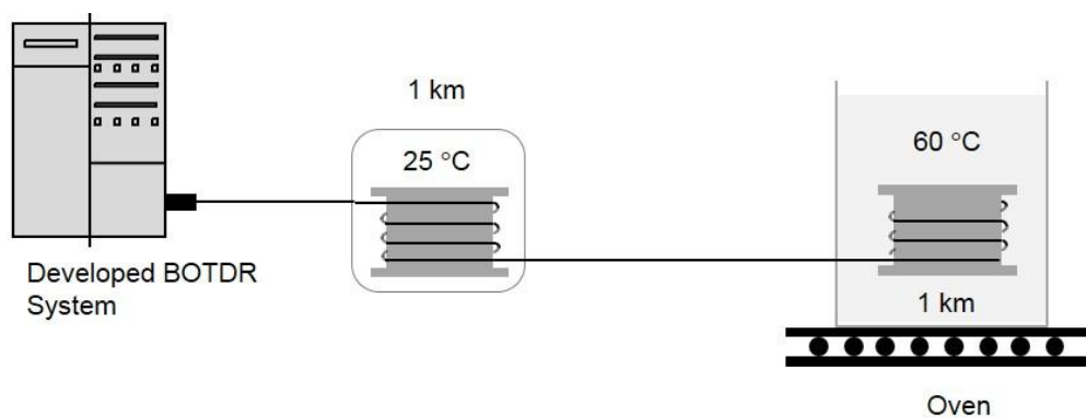
Figure 7. (a) Experimental setup and (b) comparison of FP-LD and SLED based OTDR trace for evaluating the performance.
