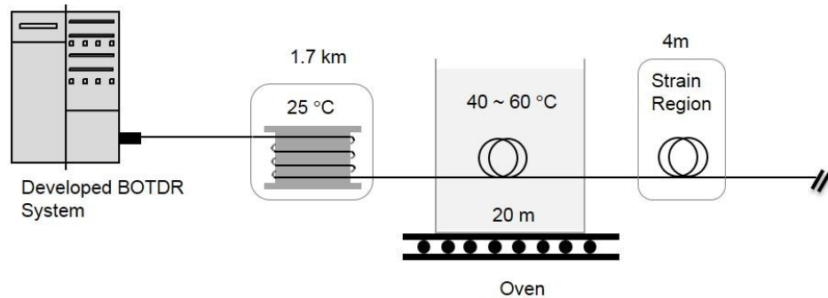
Figure 9. (a) Experimental setup for evaluating the strain measurement performance of the developed Brillouin OTDR system and (b) the result of the strain change profiles measurement.
