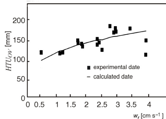
Figure 3. HTU variation with the vapour velocity w_f P = 3 bar, T = 24.68 K
