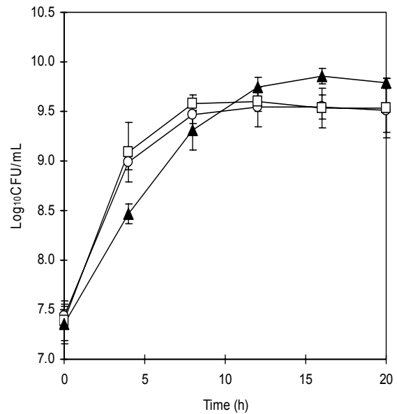
Figure 5: Growth curves of L. salivarius i 24 in MRS broth (▲), optimum-point (□) and center point (o) media as obtained from the validation experiment
