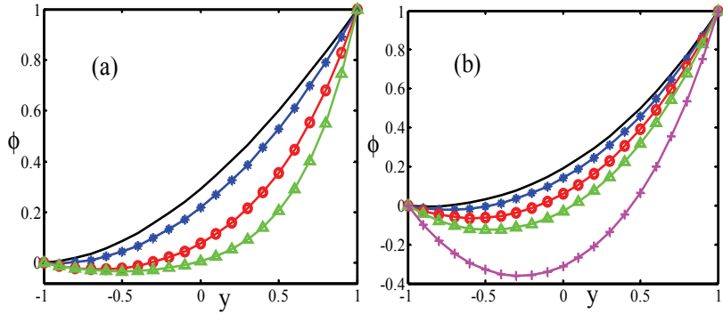
Figure 5. Concentration distribution; Re = 1 , K_1 = -1 , t = 1 , \omega = 1 , \varepsilon = 0.001 , \vartheta = 0 , \lambda x = 0.02 ; a) (-) \gamma = -0.5 , (*) \gamma = 0.5 , (O) \gamma = 1.5 , (\Delta) \gamma = 3 , Sc = 0.5 ; b) (-) Sc = 0.5 , (*) Sc = 0.6 , (O) Sc = 0.78 , (\Delta) Sc = 1 , (+) Sc = 2 , \gamma = 1 .
