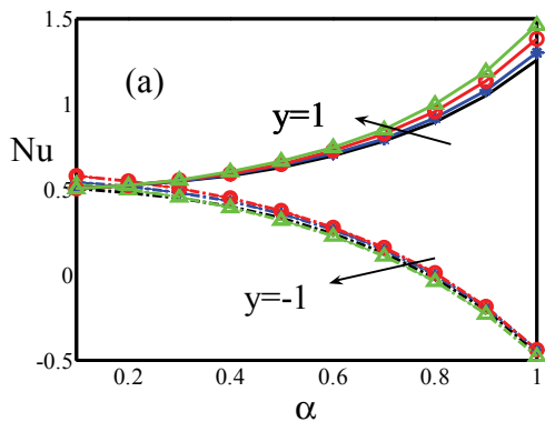
Figure 7. Nusselt number distribution; Re = 1 , t = 1 , \omega = 1 , \varepsilon = 0.3 , \lambda x = 0.02 ; a) (-) Pr = 1 , (*) Pr = 3 , (O) Pr = 5 , (\Delta) Pr = 7 , \vartheta = 0 ; b) (-) \vartheta = 0 , (*) \vartheta = \pi/8 , (O) \vartheta = \pi/4 , (\Delta) \vartheta = \pi/2 , Pr = 0.71 .
