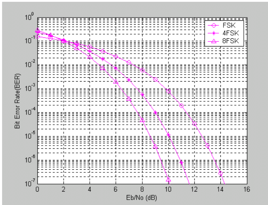
Fig. 5. MFSK Theoretical Performance.
