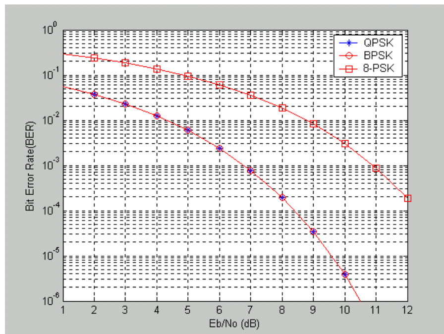
Fig. 6. MPSK Theoretical Performance.
