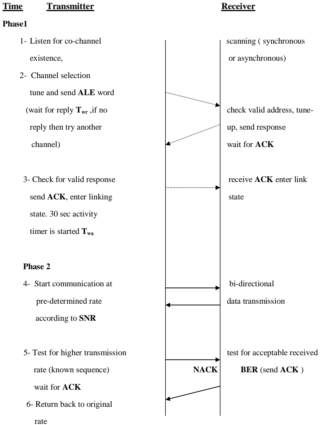
Fig. 3. Adaptation Algorithm for Point to Point.
