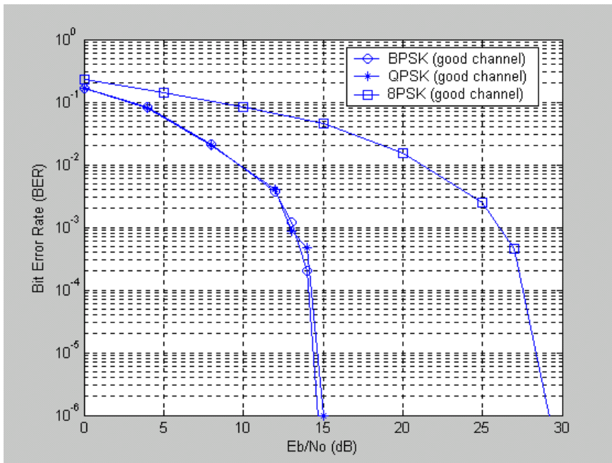
Fig. 9. MPSK Performance Over Good Channel.
