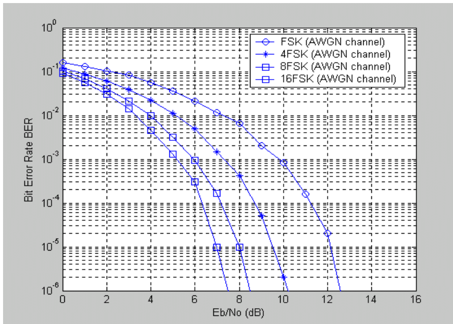
Fig. 7. MFSK Performance Over AWGN Channel (Simulated).
