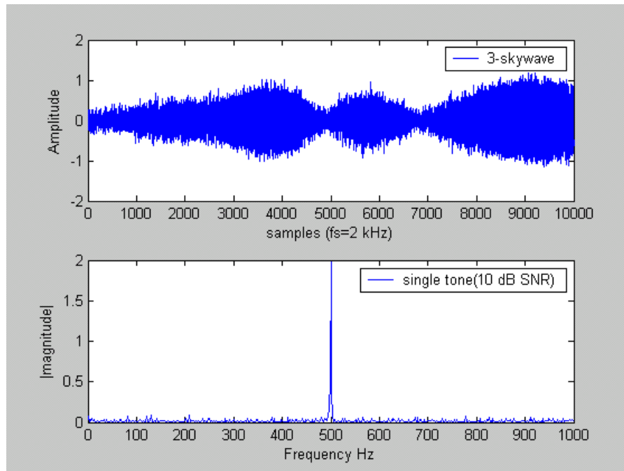
Fig. 4. Single Tone Through HF Channel.
