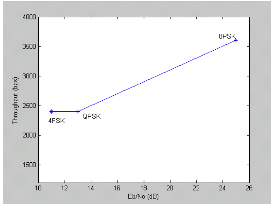
Fig. 15. HF Channel Performance.
