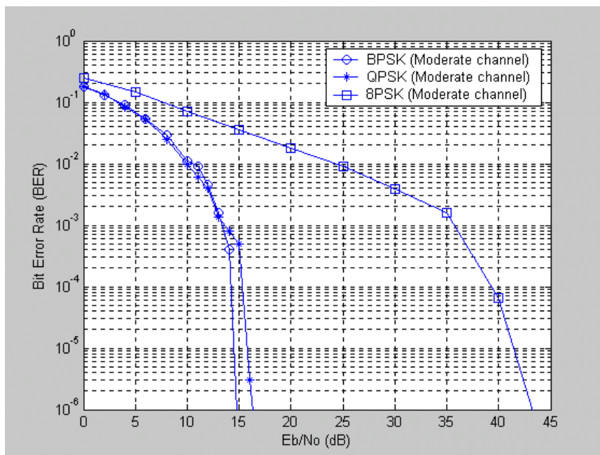
Fig. 10. MPSK Performance Over Moderate Channel.
