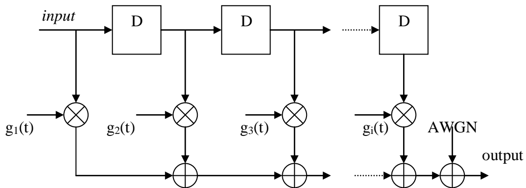
Fig. 2. Watterson HF Channel Model.
