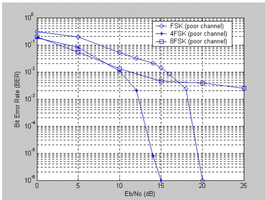
Fig. 14. MFSK Performance over Poor Channel.
