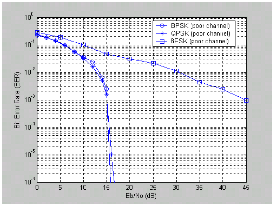
Fig. 11. MPSK Performance Over Poor Channel.
