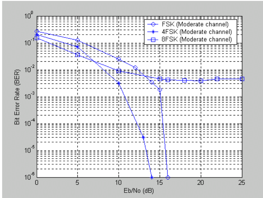
Fig. 13. MFSK Performance Over Moderate Channel.
