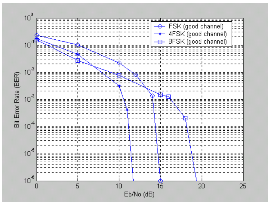
Fig. 12. MFSK Performance Over Good Channel.
