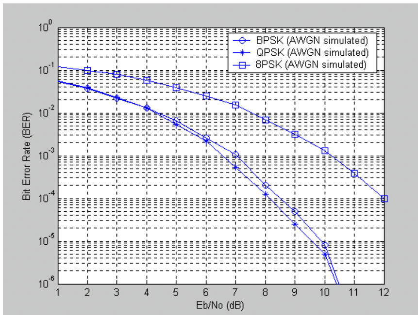
Fig. 8. MPSK Performance Over AWGN Channel (Simulated).
