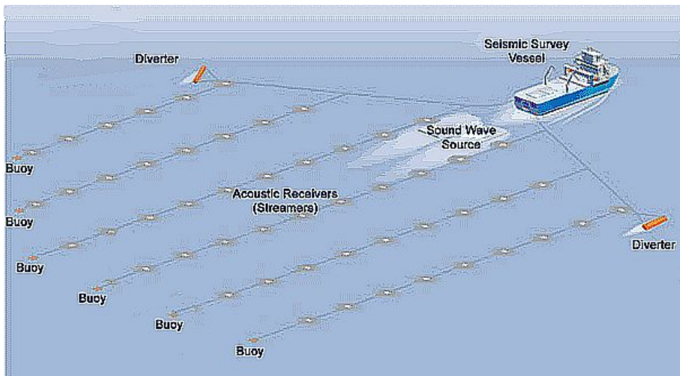
Fig. 1 Seismic research principles [5]
