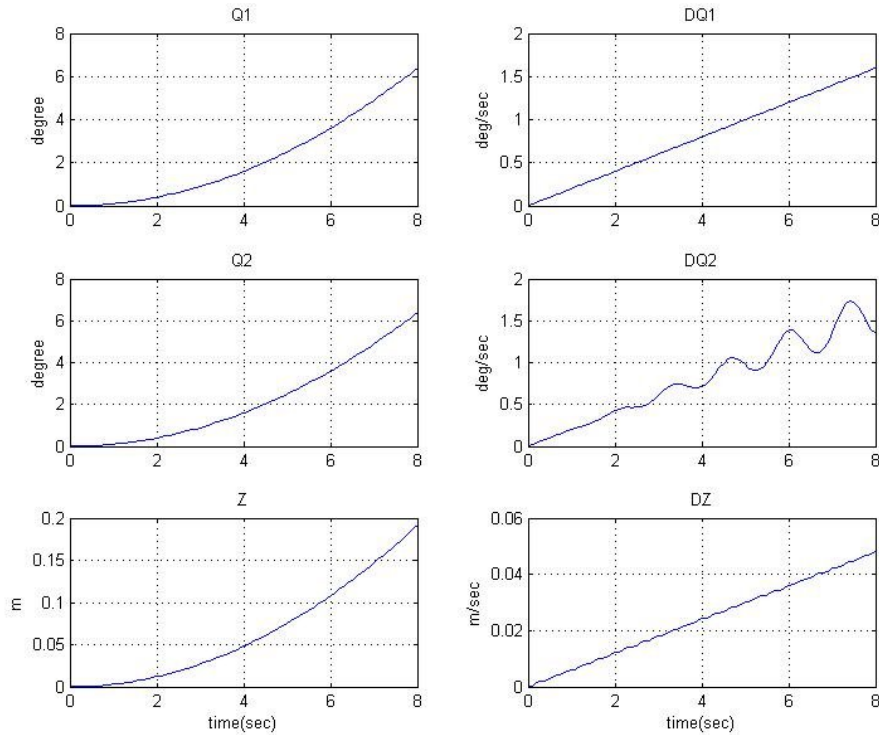
Fig.3. (b). System Response to Lifting 1000kg.
