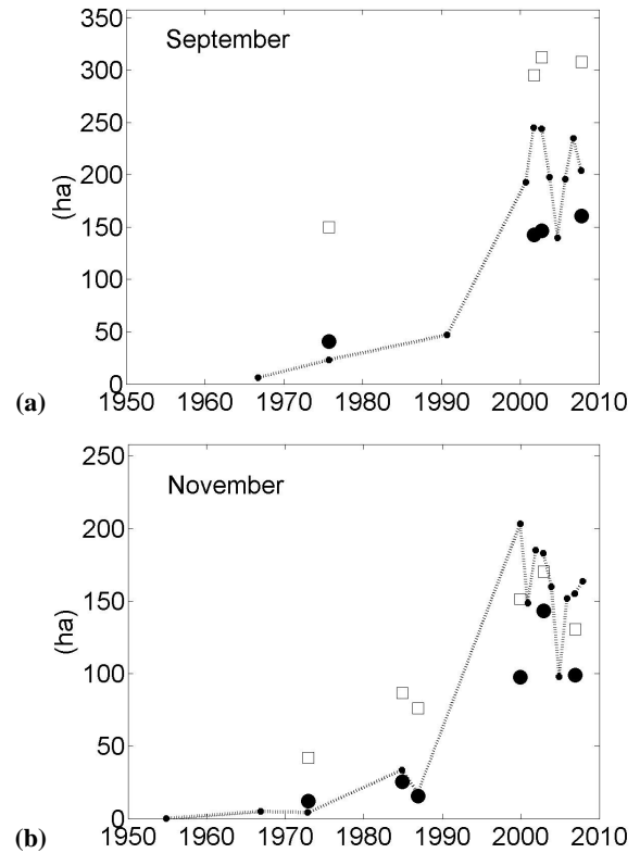
Fig. 9. (a) Average surface of water per pond (open square), average surface of turbid water (full circle) for the 91 ponds present in all September Landsat images. Also figured is the surface of the Agoufou pond in September (line), derived from all data sources. (b) Same as (a) but for November and for the 51 ponds present in all November Landsat images.
