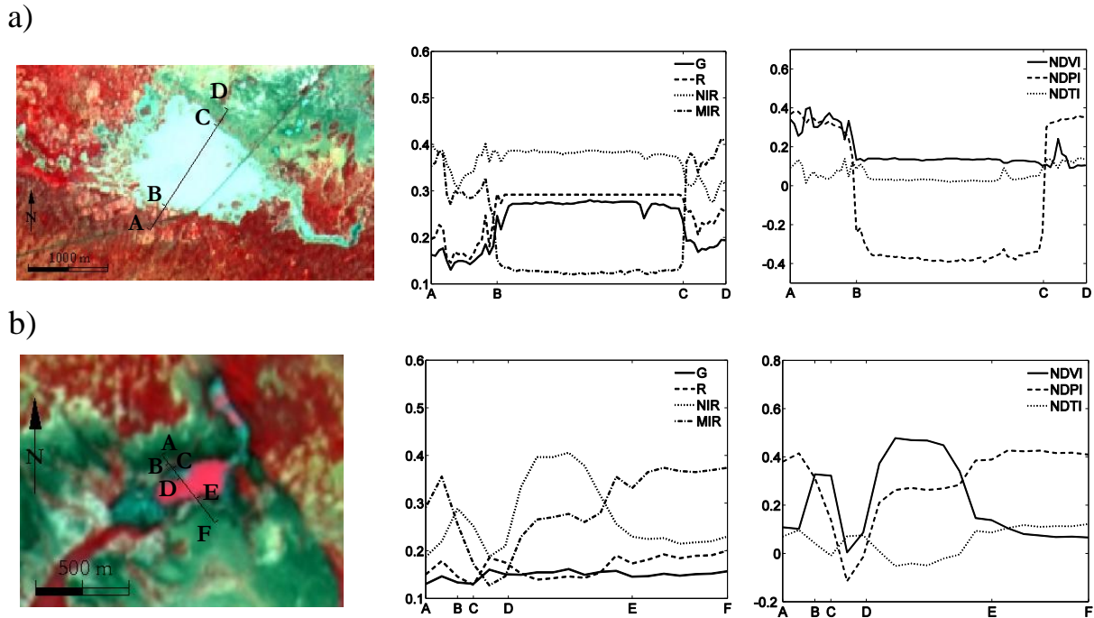
Fig. 4. From left to right, color composite, radiometric transects and corresponding indexes values for the two categories of ponds, based on a SPOT-4 image from 22 August 2005. (a) Agoufou, “blue” pond, turbid water without aquatic vegetation. A-B= vegetation on sand, B-C= open water, C-D= rocky outcrop. The broken line crossing the image (SW to NE) corresponds to the road connecting Hombori to Gossi. (b) Massi, “red” pond slightly turbid water with aquatic vegetation (center of the pond). A-B= rocky outcrop, B-C= vegetation, C-D= free water, D-E= water covered with aquatic vegetation, E-F= rocky outcrop.
