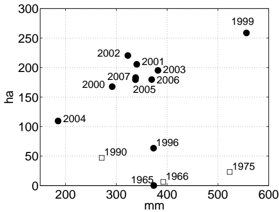
Fig. 7. Pond's area versus annual precipitations for the pond of Agoufou, October data (full circle) and September data (open square).
