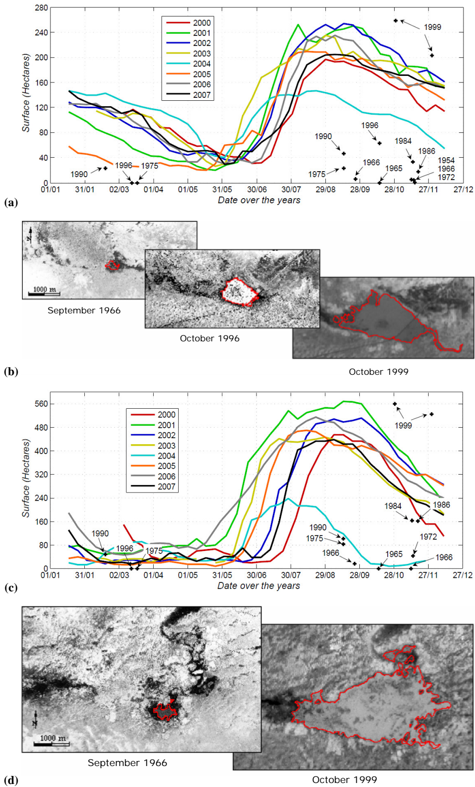
Fig. 6. Variation of the surface of Agoufou (up) and Ebang Mallam (down) over the last 50 years showing a dramatic increase. Curves are derived from MODIS data, while isolated dates come from LANDSAT, SPOT or panchromatic images. The scale is uniform throughout all images.
