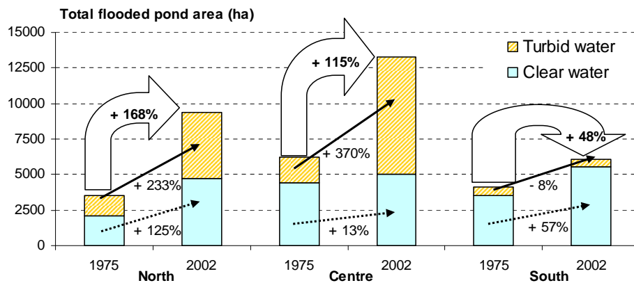
Fig. 11. Change in areas flooded with clear or turbid water (91 ponds in total) observed between 14 September 1975 and 3 September 2002 in the Gourma. Relative rates of change are calculated for the overall flood and for both clear and turbid water. Ponds are grouped following their location in the Gourma (see map in Fig. 2).
