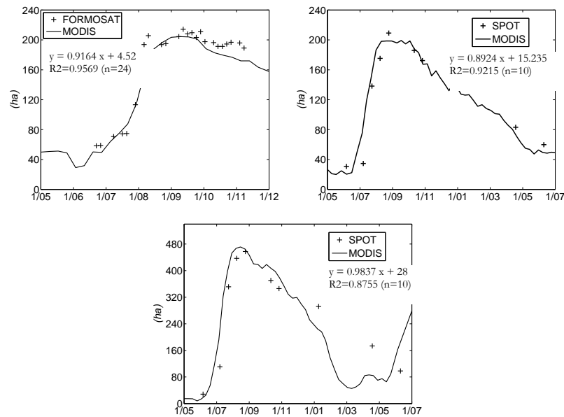
Fig. 5. Comparison of ponds' area derived from MODIS (curves) with area derived from SPOT-HRVIR and FORMOSAT-2 (point). Top is Agoufou, bottom is Ebang Mallam.
