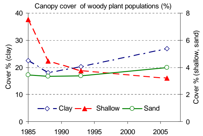
Fig. 12. Changes of the mean the canopy cover of woody populations over low-land clay soils (5 sites, left scale), dunes and low-land sandy soils (13 sites, right-scale) and eroded slopes shallow soils (4 sites, right scale) in the Gourma following the 1983–1984 drought (adapted from Hiernaux et al., 2009a).
