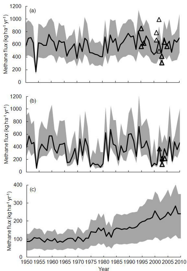
Fig. 3. Uncertainty analysis of CH 4 fluxes from marshland and rice paddies on the Sanjiang Plain.
