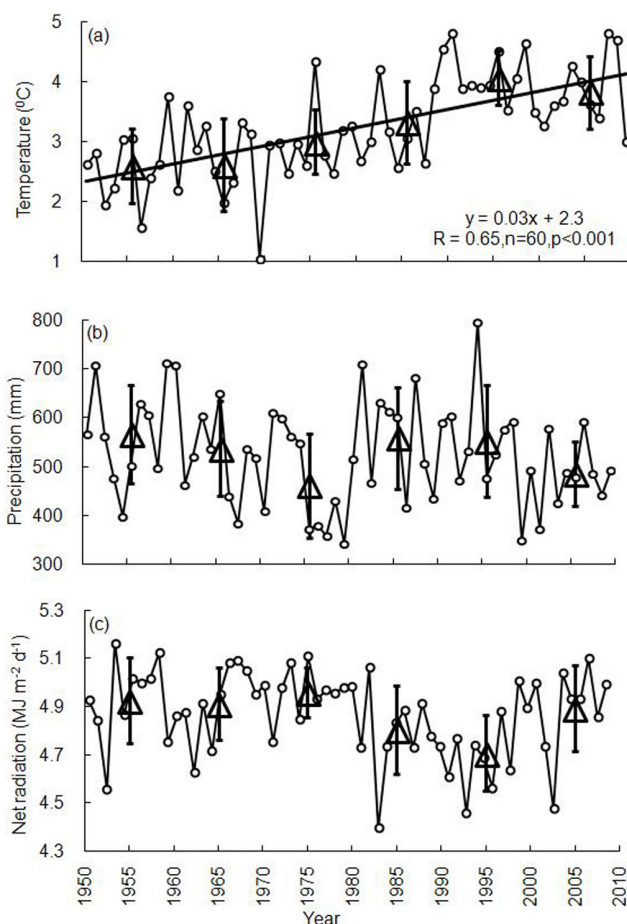
Fig. 4. Variations in the area-weighted air temperature (a), precipitation (b) and net radiation (c) on the Sanjiang Plain from 1950 to 2009. Solid lines represent the interannual variations; the triangles represent the interdecadal variations, and the vertical bars are standard deviations of 10 yr of each decade.
