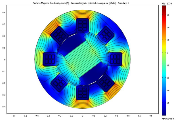
Fig. 9. Flux lines and magnetic distribution in generator with larger slot (mode 4)
