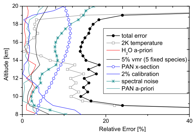
Fig. 11. Estimated total and individual relative errors in \text{PAN}_{\text{MIPAS-STR}} analysis.
