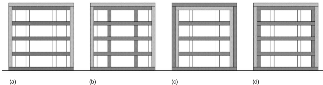
Figure 2. Concrete mass distribution; (a) low mass, (b) interior walls, (c) envelope exterior, (d) envelope interior, [diagonal hatching] concrete, [diagonal hatching] insulation, [white] no mass
