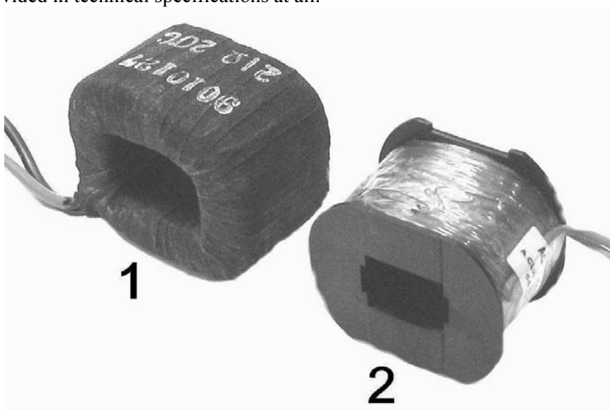
Fig. 4 – Trip coils of the CB on 160 – 170 kV from different manufacturers:
