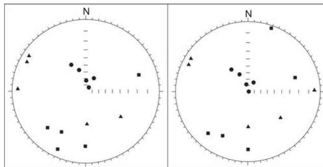
Fig. 9. Equatorial projection (on the lower hemisphere) k_{\max} (square), k_{\text{int}} (triangle) and k_{\min} (circle) of AMS ellipsoid axes for individual clay samples from the Mutalj Open Pit. Left: before correction for tectonics; right: after correction for tectonics.
