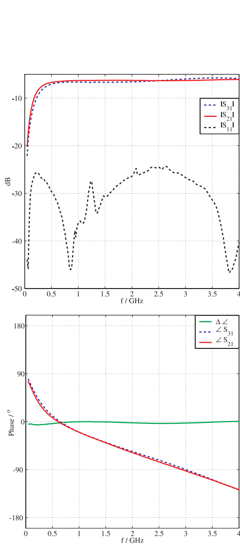
Fig. 7. Measurement results of the filter structure in Fig. 6b.
