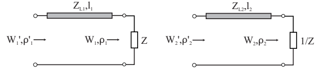
Fig. 4. Additionally inserted transmission-line-elements.
