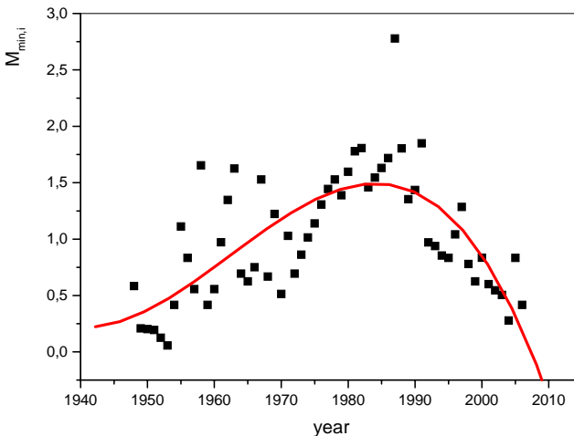
Fig. 4 Dynamics of the M_{min,i} index for Strouma River at Pernik point
