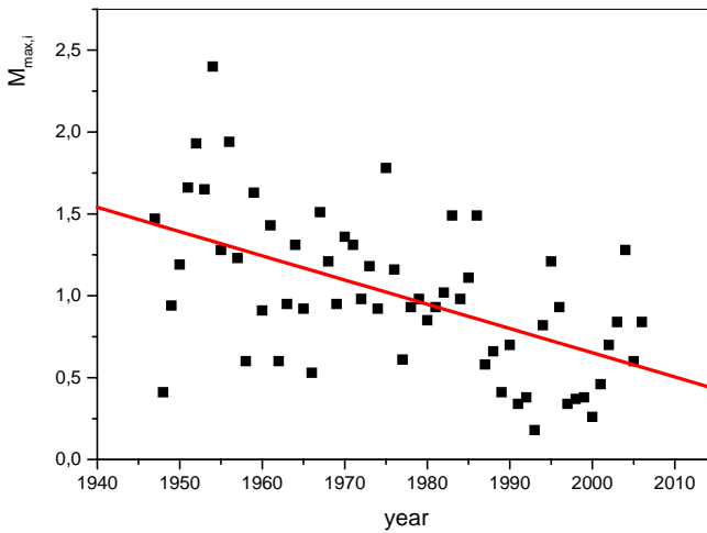
Fig. 3 Dynamics of the M_{max,i} index for Strouma River at Marino pole point
