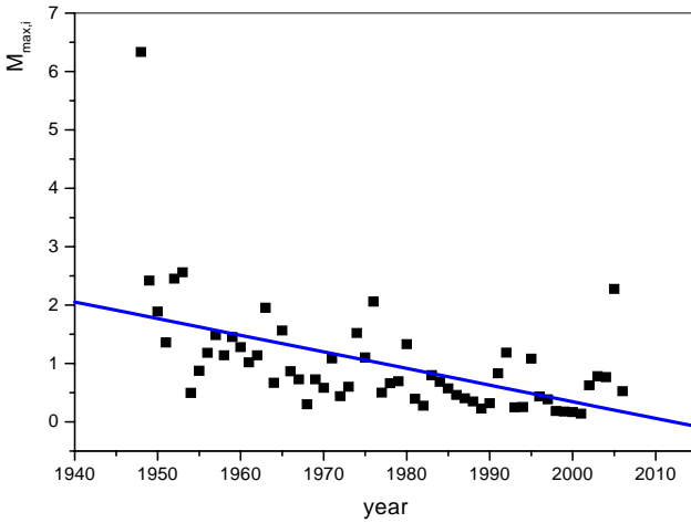
Fig. 2 Dynamics of the M_{max,i} index for Strouma River at Pernik point
