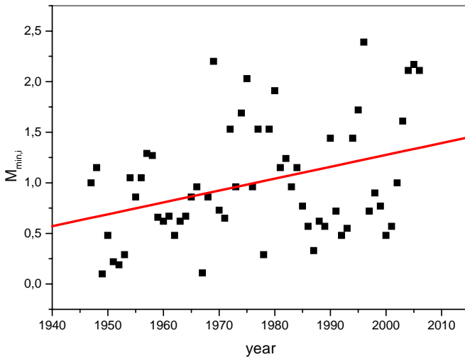
Fig. 5 Dynamics of the M_{min,i} index for Strouma River at Marino pole point
