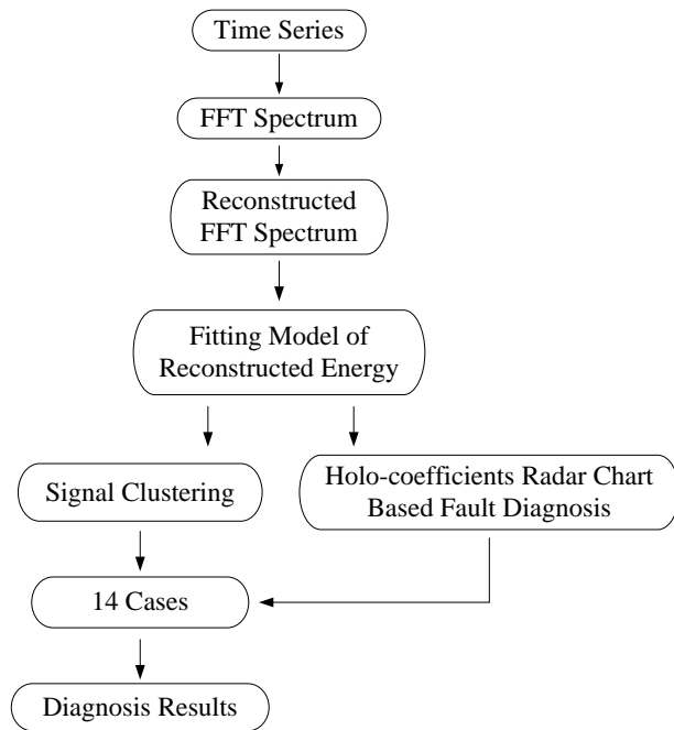
Fig.1. Overview of information reconstruction method
