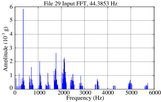
Fig.4. Reconstructed FFT spectrum of File-29
