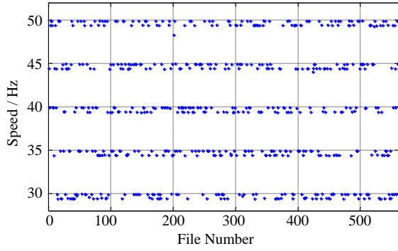
Fig.5. Input shaft speeds
