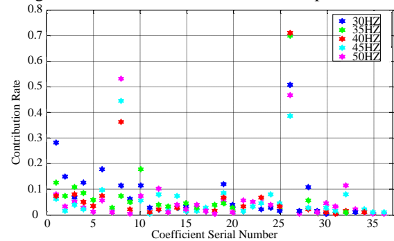
Fig.14. Holo-coefficients map of pattern B
