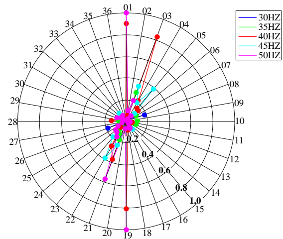
Fig.13. Holo-coefficients radar chart of pattern A
