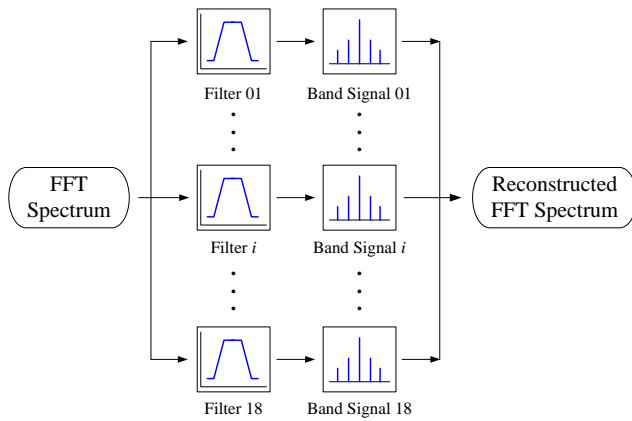
Fig.2. FFT spectrum reconstruction
