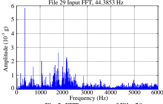
Fig.3. FFT spectrum of File-29
