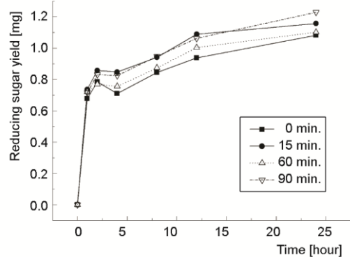
Figure 6. Reducing sugar yield of enzymatic hydrolysis with different processing time
