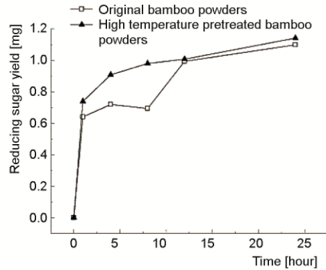
Figure 4. Reducing sugar yield of enzymatic hydrolysis on bamboo of different pretreatment
