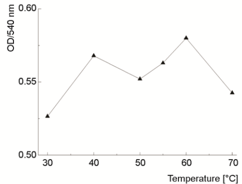
Figure 2. Effect of temperature on activities of cellulase
